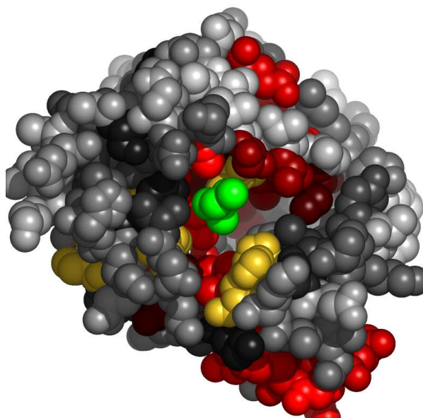
Fig. 4. Residues in 103mA, at the interface with n-butyl isocyanide, colored by their relative importance. The ligand (n-butyl isocyanide) is colored green. Atoms further than 30Å away from the geometric center of the ligand, as well as on the line of sight to the ligand were removed. (See Appendix for the coloring scheme for the protein chain 103mA.)
