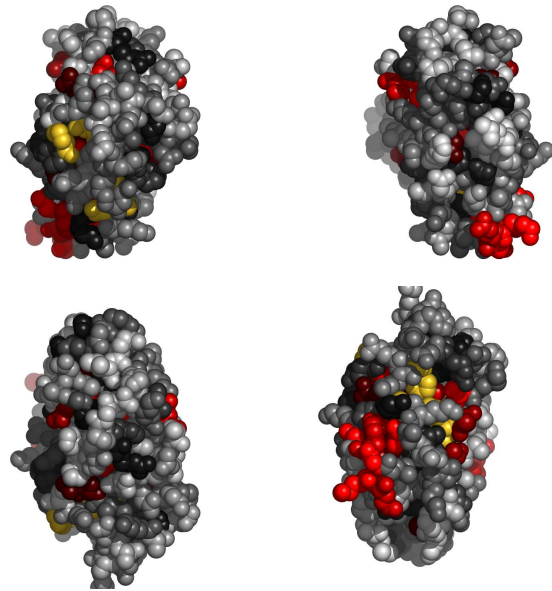
Fig. 2. Residues in 103mA, colored by their relative importance. Clockwise: front, back, top and bottom views.
