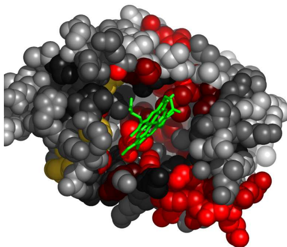
Fig. 5. Residues in 103mA, at the interface with HEM, colored by their relative importance. The ligand (HEM) is colored green. Atoms further than 30 Å away from the geometric center of the ligand, as well as on the line of sight to the ligand were removed. (See Appendix for the coloring scheme for the protein chain 103mA.)
