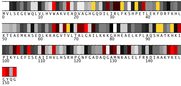
Fig. 1. Residues 0-153 in 103mA colored by their relative importance. (See Appendix, Fig.7, for the coloring scheme.)
