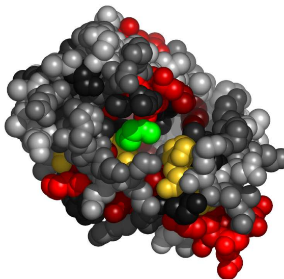
Fig. 5. Residues in 111mA, at the interface with n-butyl isocyanide, colored by their relative importance. The ligand (n-butyl isocyanide) is colored green. Atoms further than 30Å away from the geometric center of the ligand, as well as on the line of sight to the ligand were removed. (See Appendix for the coloring scheme for the protein chain 111mA.)
