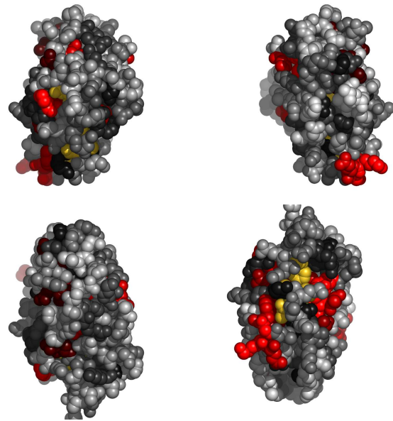
Fig. 2. Residues in 111mA, colored by their relative importance. Clockwise: front, back, top and bottom views.
