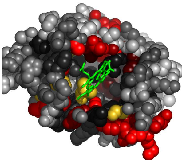
Fig. 4. Residues in 111mA, at the interface with HEM, colored by their relative importance. The ligand (HEM) is colored green. Atoms further than 30Å away from the geometric center of the ligand, as well as on the line of sight to the ligand were removed. (See Appendix for the coloring scheme for the protein chain 111mA.)
