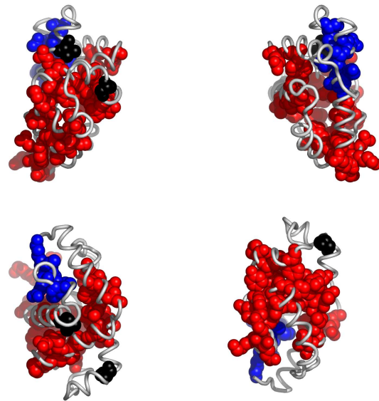
Fig. 3. Residues in 111mA, colored according to the cluster they belong to: red, followed by blue and yellow are the largest clusters (see Appendix for the coloring scheme). Clockwise: front, back, top and bottom views. The corresponding Pymol script is attached.
