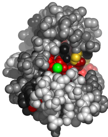
Fig. 4. Residues in 1261A, at the interface with chloride ion, colored by their relative importance. The ligand (chloride ion) is colored green. Atoms further than 30Å away from the geometric center of the ligand, as well as on the line of sight to the ligand were removed. (See Appendix for the coloring scheme for the protein chain 1261A.)
