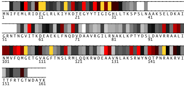
Fig. 1. Residues 1-162 in 1281A colored by their relative importance. (See Appendix, Fig.6, for the coloring scheme.)
