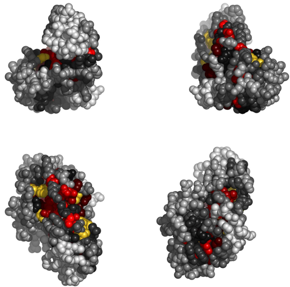
Fig. 2. Residues in 1281A, colored by their relative importance. Clockwise: front, back, top and bottom views.
