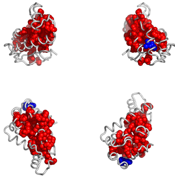
Fig. 3. Residues in 1281A, colored according to the cluster they belong to: red, followed by blue and yellow are the largest clusters (see Appendix for the coloring scheme). Clockwise: front, back, top and bottom views. The corresponding Pymol script is attached.
