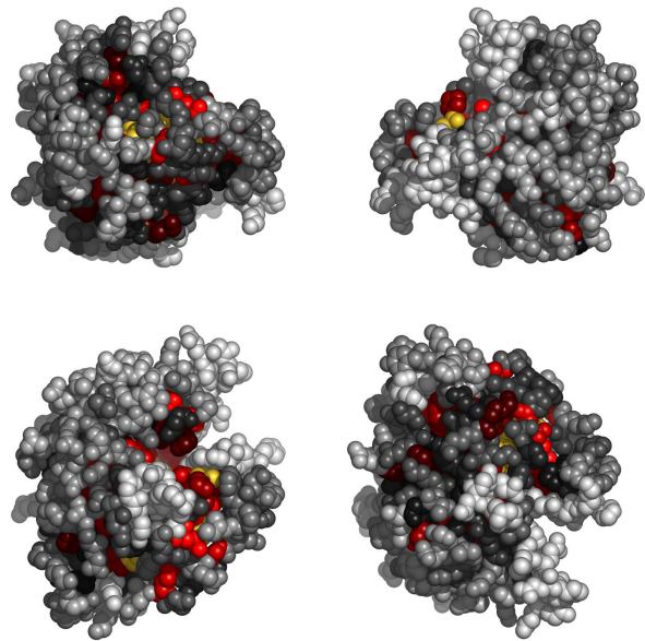
Fig. 3. Residues in 12caA, colored by their relative importance. Clockwise: front, back, top and bottom views.
