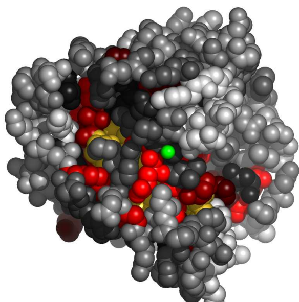
Fig. 5. Residues in 12caA, at the interface with mercury (ii) ion, colored by their relative importance. The ligand (mercury (ii) ion) is colored green. Atoms further than 30Å away from the geometric center of the ligand, as well as on the line of sight to the ligand were removed. (See Appendix for the coloring scheme for the protein chain 12caA.)
