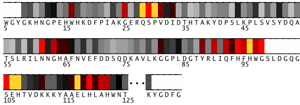
Fig. 1. Residues 5-132 in 12caA colored by their relative importance. (See Appendix, Fig.7, for the coloring scheme.)
