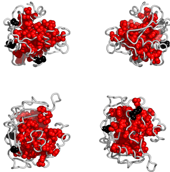
Fig. 4. Residues in 12caA, colored according to the cluster they belong to: red, followed by blue and yellow are the largest clusters (see Appendix for the coloring scheme). Clockwise: front, back, top and bottom views. The corresponding Pymol script is attached.
