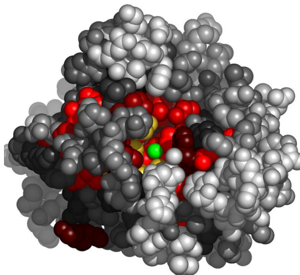
Fig. 5. Residues in 12caA, at the interface with mercury (ii) ion, colored by their relative importance. The ligand (mercury (ii) ion) is colored green. Atoms further than 30Å away from the geometric center of the ligand, as well as on the line of sight to the ligand were removed. (See Appendix for the coloring scheme for the protein chain 12caA.)
