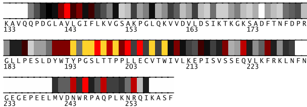
Fig. 2. Residues 133-260 in 12caA colored by their relative importance. (See Appendix, Fig.7, for the coloring scheme.)
