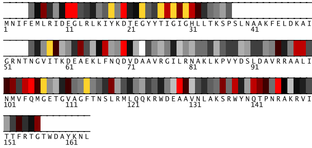
Fig. 1. Residues 1-164 in 1371B colored by their relative importance. (See Appendix, Fig.5, for the coloring scheme.)
