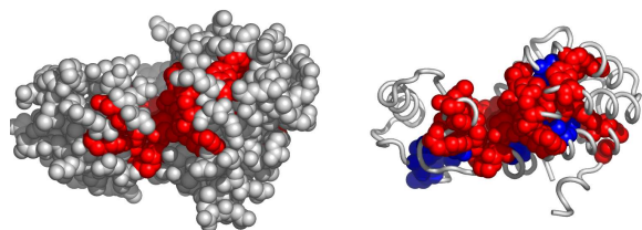
Fig. 4. A possible active surface on the chain 1371B. The larger cluster it belongs to is shown in blue.
