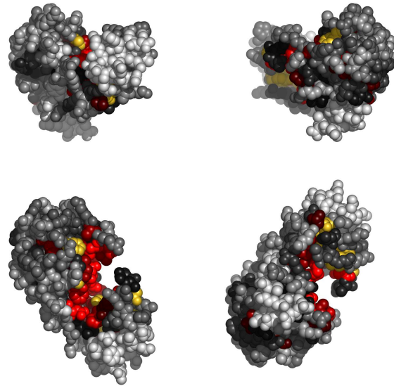
Fig. 2. Residues in 1371B, colored by their relative importance. Clockwise: front, back, top and bottom views.
