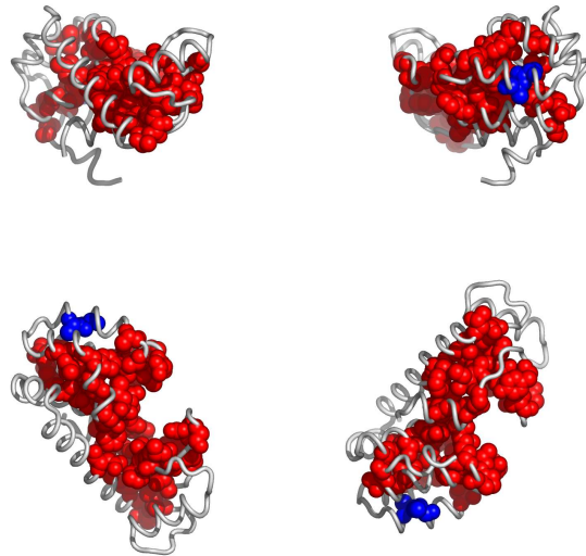
Fig. 3. Residues in 1371B, colored according to the cluster they belong to: red, followed by blue and yellow are the largest clusters (see Appendix for the coloring scheme). Clockwise: front, back, top and bottom views. The corresponding Pymol script is attached.
