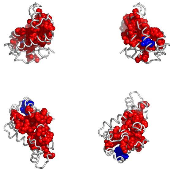
Fig. 3. Residues in 1451A, colored according to the cluster they belong to: red, followed by blue and yellow are the largest clusters (see Appendix for the coloring scheme). Clockwise: front, back, top and bottom views. The corresponding Pymol script is attached.
