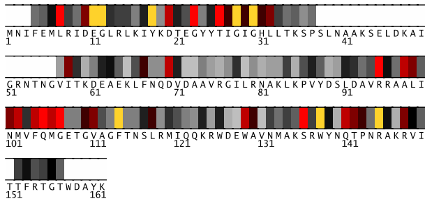
Fig. 1. Residues 1-162 in 1451A colored by their relative importance. (See Appendix, Fig.5, for the coloring scheme.)
