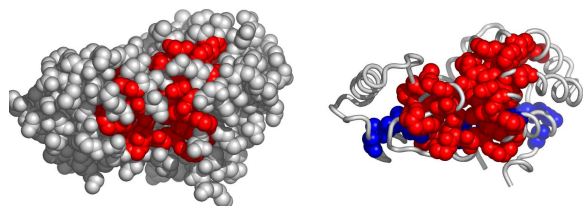
Fig. 4. A possible active surface on the chain 1451A. The larger cluster it belongs to is shown in blue.
