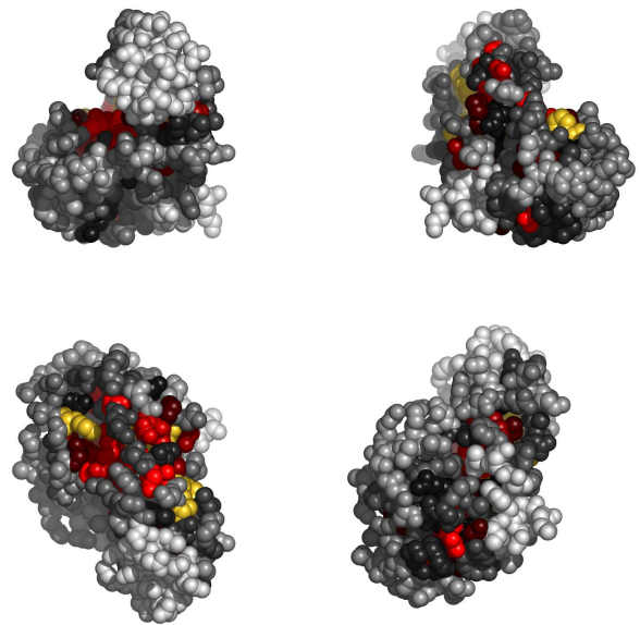
Fig. 2. Residues in 1451A, colored by their relative importance. Clockwise: front, back, top and bottom views.
