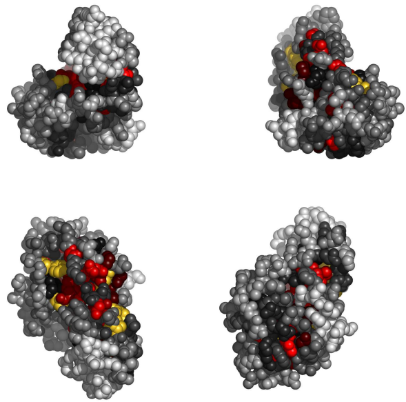
Fig. 2. Residues in 1651A, colored by their relative importance. Clockwise: front, back, top and bottom views.
