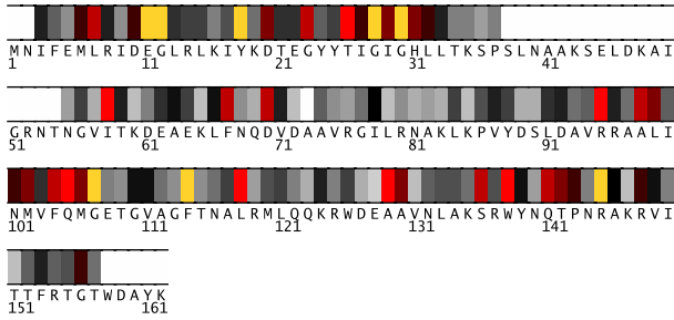
Fig. 1. Residues 1-162 in 1651A colored by their relative importance. (See Appendix, Fig.7, for the coloring scheme.)
