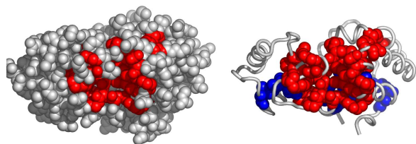
Fig. 6. A possible active surface on the chain 1651A. The larger cluster it belongs to is shown in blue.
