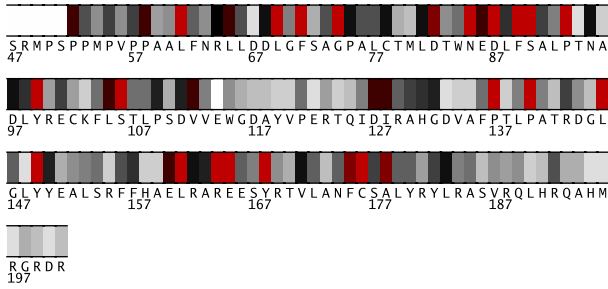
Fig. 1. Residues 47-201 in 16vpA colored by their relative importance. (See Appendix, Fig.8, for the coloring scheme.)
