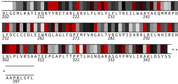
Fig. 2. Residues 202-402 in 16vpA colored by their relative importance. (See Appendix, Fig.8, for the coloring scheme.)
