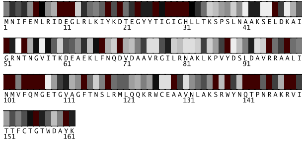
Fig. 1. Residues 1-162 in 1771A colored by their relative importance. (See Appendix, Fig.5, for the coloring scheme.)
