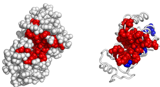
Fig. 4. A possible active surface on the chain 1771A. The larger cluster it belongs to is shown in blue.
