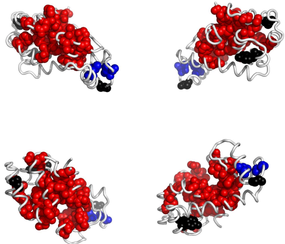
Fig. 3. Residues in 1771A, colored according to the cluster they belong to: red, followed by blue and yellow are the largest clusters (see Appendix for the coloring scheme). Clockwise: front, back, top and bottom views. The corresponding Pymol script is attached.
