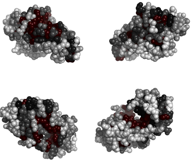
Fig. 2. Residues in 1771A, colored by their relative importance. Clockwise: front, back, top and bottom views.
