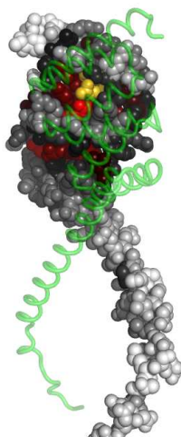
Fig. 6. Residues in 1a17A, at the interface with 1a17A3, colored by their relative importance. 1a17A3 is shown in backbone representation (See Appendix for the coloring scheme for the protein chain 1a17A.)
