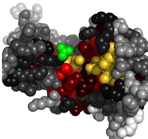
Fig. 5. Residues in 1a17A, at the interface with sulfate ion, colored by their relative importance. The ligand (sulfate ion) is colored green. Atoms further than 30Å away from the geometric center of the ligand, as well as on the line of sight to the ligand were removed. (See Appendix for the coloring scheme for the protein chain 1a17A.)
