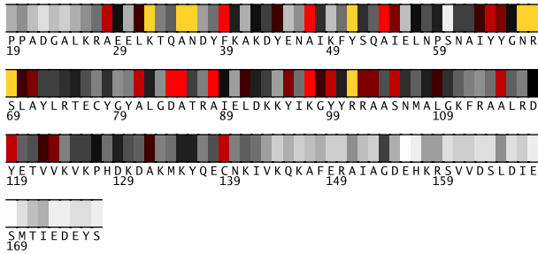
Fig. 1. Residues 19-177 in 1a17A colored by their relative importance. (See Appendix, Fig.8, for the coloring scheme.)
