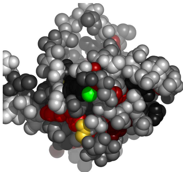
Fig. 9. Residues in 1a29A, at the interface with calcium ion, colored by their relative importance. The ligand (calcium ion) is colored green. Atoms further than 30Å away from the geometric center of the ligand, as well as on the line of sight to the ligand were removed. (See Appendix for the coloring scheme for the protein chain 1a29A.)
