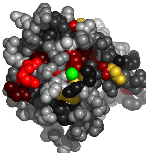
Fig. 7. Residues in 1a29A, at the interface with calcium ion, colored by their relative importance. The ligand (calcium ion) is colored green. Atoms further than 30Å away from the geometric center of the ligand, as well as on the line of sight to the ligand were removed. (See Appendix for the coloring scheme for the protein chain 1a29A.)
