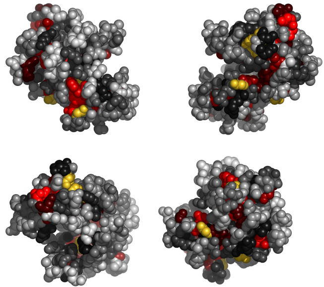
Fig. 2. Residues in 1a29A, colored by their relative importance. Clockwise: front, back, top and bottom views.
