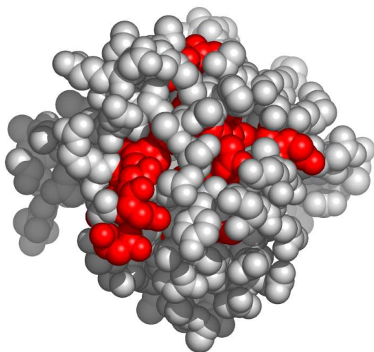
Fig. 11. Another possible active surface on the chain 1a29A.
