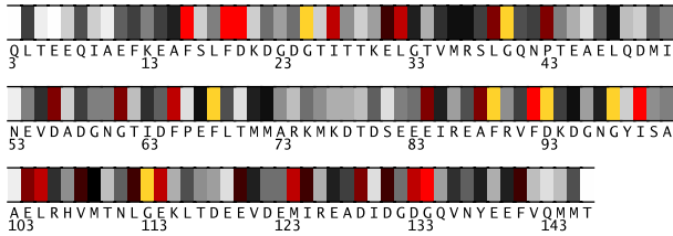
Fig. 1. Residues 3-146 in 1a29A colored by their relative importance. (See Appendix, Fig.12, for the coloring scheme.)
