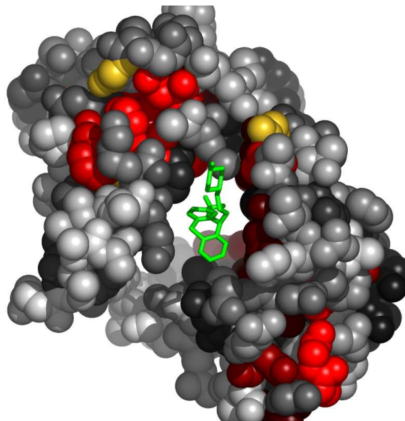
Fig. 8. Residues in 1a29A, at the interface with TFP, colored by their relative importance. The ligand (TFP) is colored green. Atoms further than 30Å away from the geometric center of the ligand, as well as on the line of sight to the ligand were removed. (See Appendix for the coloring scheme for the protein chain 1a29A.)
