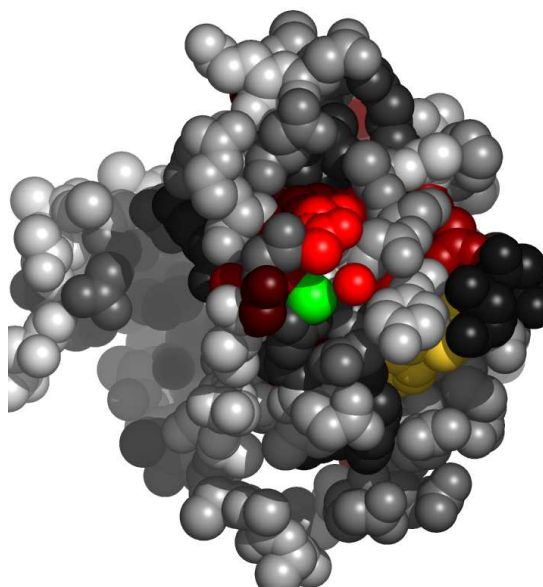
Fig. 4. Residues in 1a29A, at the interface with calcium ion, colored by their relative importance. The ligand (calcium ion) is colored green. Atoms further than 30Å away from the geometric center of the ligand, as well as on the line of sight to the ligand were removed. (See Appendix for the coloring scheme for the protein chain 1a29A.)
