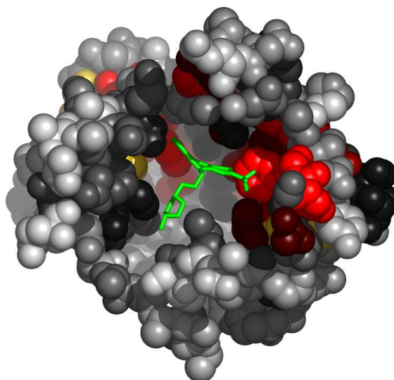
Fig. 5. Residues in 1a29A, at the interface with TFP, colored by their relative importance. The ligand (TFP) is colored green. Atoms further than 30Å away from the geometric center of the ligand, as well as on the line of sight to the ligand were removed. (See Appendix for the coloring scheme for the protein chain 1a29A.)
