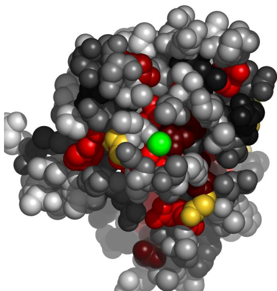
Fig. 6. Residues in 1a29A, at the interface with calcium ion, colored by their relative importance. The ligand (calcium ion) is colored green. Atoms further than 30Å away from the geometric center of the ligand, as well as on the line of sight to the ligand were removed. (See Appendix for the coloring scheme for the protein chain 1a29A.)
