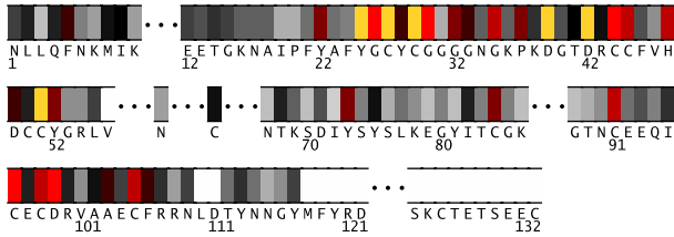
Fig. 1. Residues 1-133 in 1a2aF colored by their relative importance. (See Appendix, Fig.8, for the coloring scheme.)
