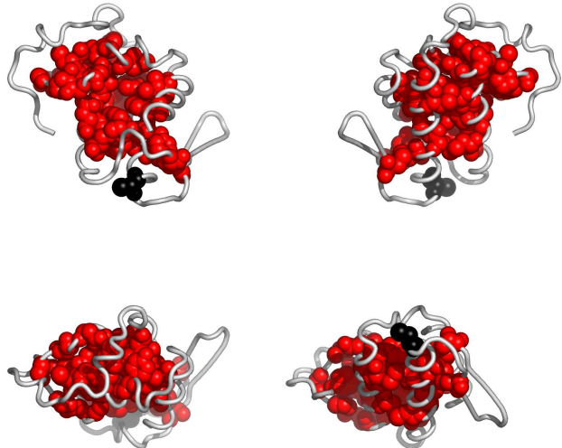
Fig. 2. Residues in 1a2aF, colored by their relative importance. Clockwise: front, back, top and bottom views.
