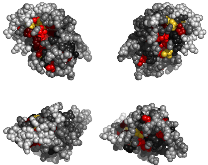
Fig. 1. Residues 1-133 in 1a2aF colored by their relative importance. (See Appendix, Fig.8, for the coloring scheme.)
