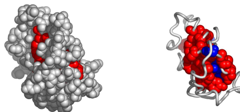
Fig. 7. A possible active surface on the chain 1a2aF. The larger cluster it belongs to is shown in blue.
