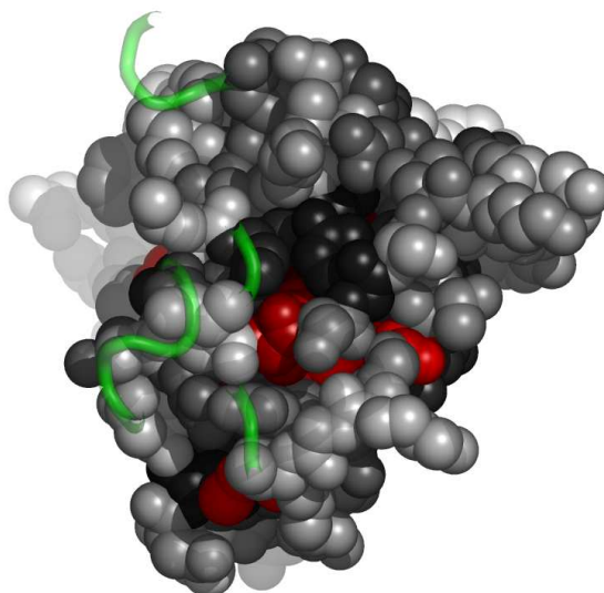
Fig. 6. Residues in 1a2aF, at the interface with 1a2aG, colored by their relative importance. 1a2aG is shown in backbone representation (See Appendix for the coloring scheme for the protein chain 1a2aF.)
