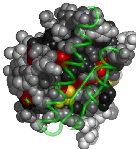
Fig. 4. Residues in 1a2aF, at the interface with 1a2aH, colored by their relative importance. 1a2aH is shown in backbone representation (See Appendix for the coloring scheme for the protein chain 1a2aF.)
