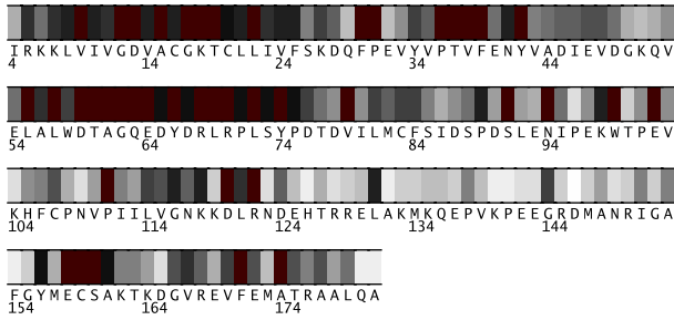
Fig. 1. Residues 4-181 in 1a2bA colored by their relative importance. (See Appendix, Fig.6, for the coloring scheme.)
