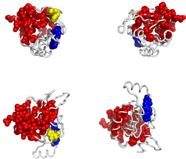
Fig. 3. Residues in 1a2bA, colored according to the cluster they belong to: red, followed by blue and yellow are the largest clusters (see Appendix for the coloring scheme). Clockwise: front, back, top and bottom views. The corresponding Pymol script is attached.
