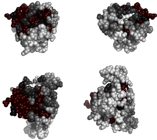
Fig. 2. Residues in 1a2bA, colored by their relative importance. Clockwise: front, back, top and bottom views.
