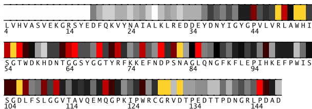
Fig. 1. Residues 4-148 in 1a2fA colored by their relative importance. (See Appendix, Fig.7, for the coloring scheme.)
