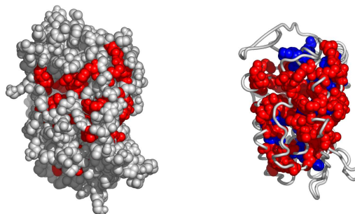
Fig. 6. A possible active surface on the chain 1a2fA. The larger cluster it belongs to is shown in blue.
