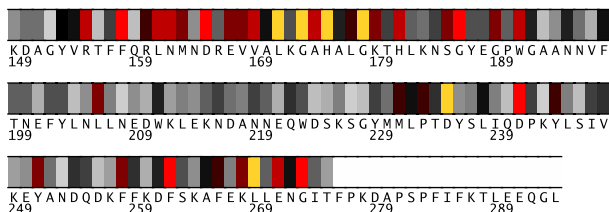
Fig. 2. Residues 149-294 in 1a2fA colored by their relative importance. (See Appendix, Fig.7, for the coloring scheme.)
