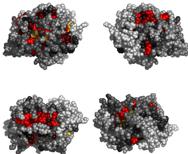
Fig. 2. Residues 149-294 in 1a2fA colored by their relative importance. (See Appendix, Fig.7, for the coloring scheme.)
