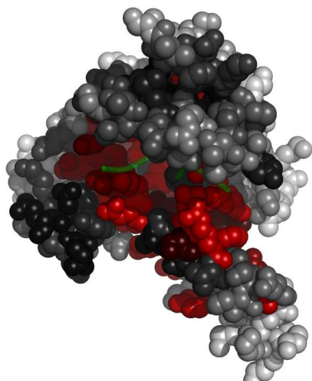
Fig. 5. Residues in 1a37A, at the interface with 1a37P, colored by their relative importance. 1a37P is shown in backbone representation (See Appendix for the coloring scheme for the protein chain 1a37A.)
