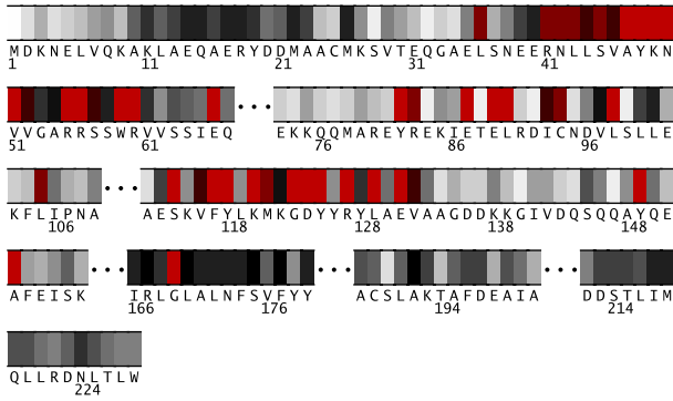
Fig. 1. Residues 1-228 in 1a37A colored by their relative importance. (See Appendix, Fig.7, for the coloring scheme.)
