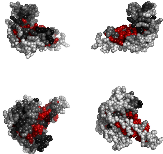
Fig. 2. Residues in 1a37A, colored by their relative importance. Clockwise: front, back, top and bottom views.
