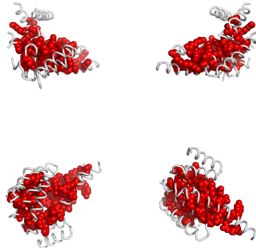
Fig. 3. Residues in 1a37A, colored according to the cluster they belong to: red, followed by blue and yellow are the largest clusters (see Appendix for the coloring scheme). Clockwise: front, back, top and bottom views. The corresponding Pymol script is attached.
