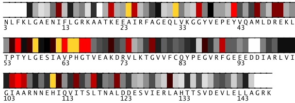
Fig. 1. Residues 3-148 in 1a3aC colored by their relative importance. (See Appendix, Fig.6, for the coloring scheme.)
