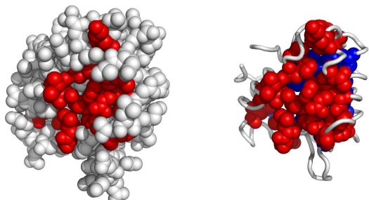
Fig. 5. A possible active surface on the chain 1a3aC. The larger cluster it belongs to is shown in blue.
