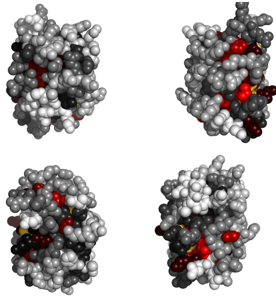
Fig. 2. Residues in 1a3aC, colored by their relative importance. Clockwise: front, back, top and bottom views.
