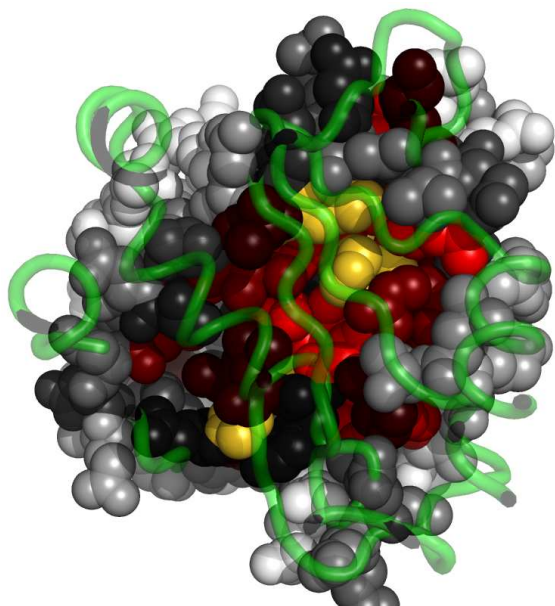
Fig. 4. Residues in 1a3aC, at the interface with 1a3aD, colored by their relative importance. 1a3aD is shown in backbone representation (See Appendix for the coloring scheme for the protein chain 1a3aC.)
