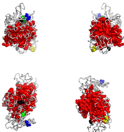
Fig. 4. Residues in 1a3wA, colored according to the cluster they belong to: red, followed by blue and yellow are the largest clusters (see Appendix for the coloring scheme). Clockwise: front, back, top and bottom views. The corresponding Pymol script is attached.
