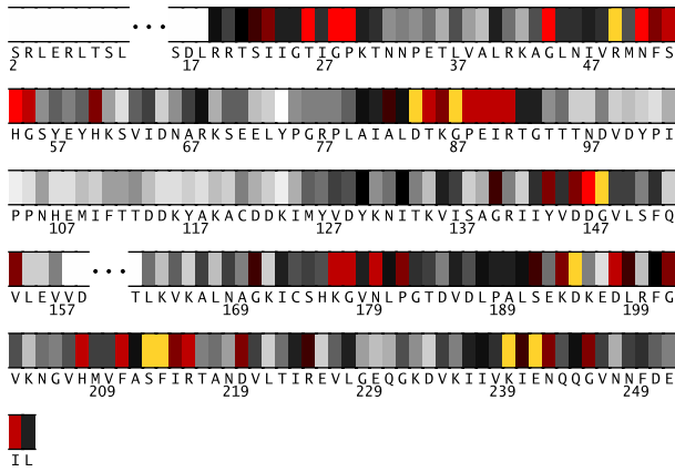
Fig. 1. Residues 2-254 in 1a3wA colored by their relative importance. (See Appendix, Fig.11, for the coloring scheme.)
