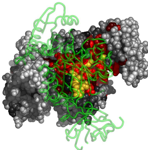
Fig. 10. Residues in 1a3wA, at the interface with 1a3wB, colored by their relative importance. 1a3wB is shown in backbone representation (See Appendix for the coloring scheme for the protein chain 1a3wA.)
