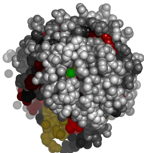
Fig. 5. Residues in 1a3wA, at the interface with manganese (ii) ion, colored by their relative importance. The ligand (manganese (ii) ion) is colored green. Atoms further than 30 Å away from the geometric center of the ligand, as well as on the line of sight to the ligand were removed. (See Appendix for the coloring scheme for the protein chain 1a3wA.)
