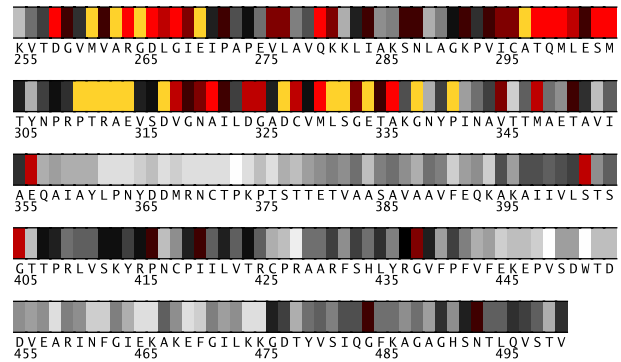
Fig. 2. Residues 255-500 in 1a3wA colored by their relative importance. (See Appendix, Fig.11, for the coloring scheme.)
