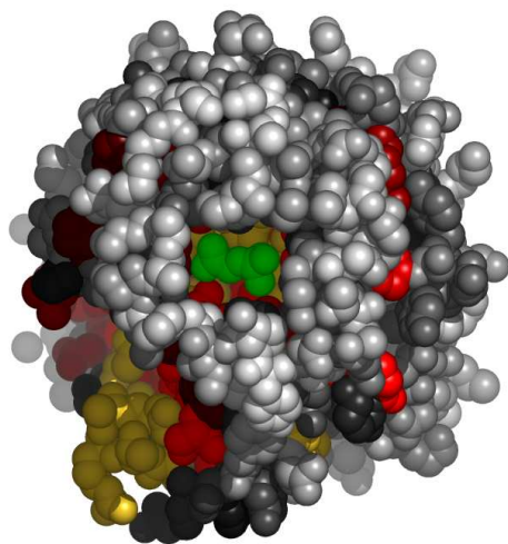
Fig. 7. Residues in 1a3wA, at the interface with PGA, colored by their relative importance. The ligand (PGA) is colored green. Atoms further than 30Å away from the geometric center of the ligand, as well as on the line of sight to the ligand were removed. (See Appendix for the coloring scheme for the protein chain 1a3wA.)
