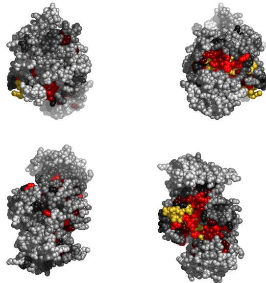
Fig. 3. Residues in 1a3wA, colored by their relative importance. Clockwise: front, back, top and bottom views.
