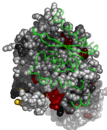
Fig. 6. Residues in 1a3wA, at the interface with 1a3wA1, colored by their relative importance. 1a3wA1 is shown in backbone representation (See Appendix for the coloring scheme for the protein chain 1a3wA.)
