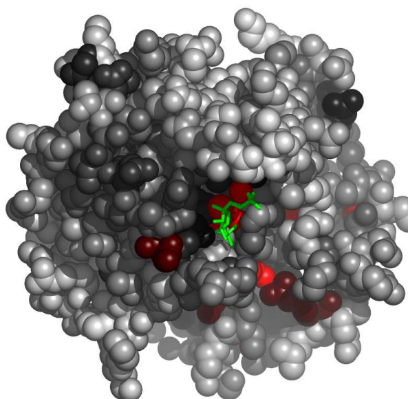
Fig. 8. Residues in 1a3wA, at the interface with FBP, colored by their relative importance. The ligand (FBP) is colored green. Atoms further than 30Å away from the geometric center of the ligand, as well as on the line of sight to the ligand were removed. (See Appendix for the coloring scheme for the protein chain 1a3wA.)
