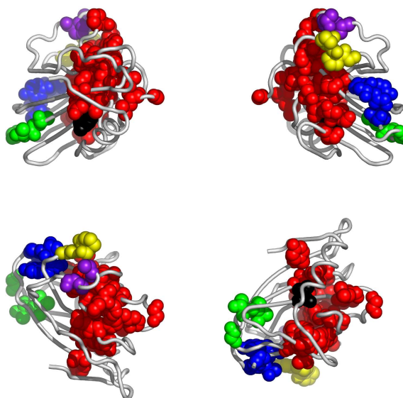
Fig. 3. Residues in 1a3zA, colored according to the cluster they belong to: red, followed by blue and yellow are the largest clusters (see Appendix for the coloring scheme). Clockwise: front, back, top and bottom views. The corresponding Pymol script is attached.
