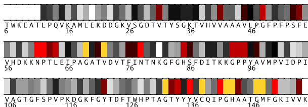
Fig. 1. Residues 6-155 in 1a3zA colored by their relative importance. (See Appendix, Fig.6, for the coloring scheme.)
