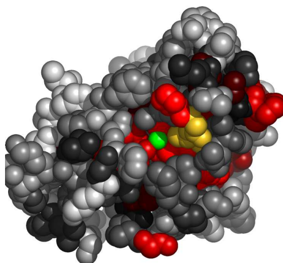
Fig. 4. Residues in 1a3zA, at the interface with copper (i) ion, colored by their relative importance. The ligand (copper (i) ion) is colored green. Atoms further than 30 Å away from the geometric center of the ligand, as well as on the line of sight to the ligand were removed. (See Appendix for the coloring scheme for the protein chain 1a3zA.)
