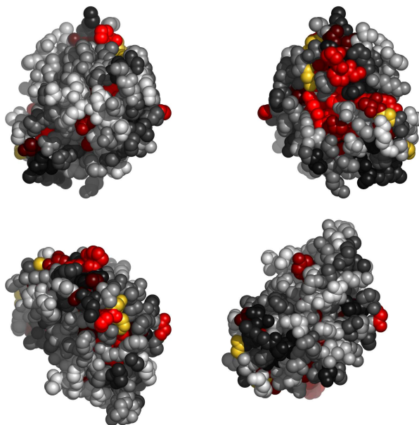
Fig. 2. Residues in 1a3zA, colored by their relative importance. Clockwise: front, back, top and bottom views.
