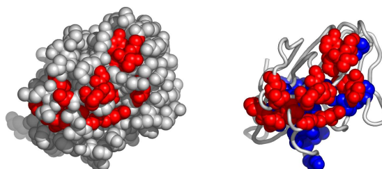
Fig. 5. A possible active surface on the chain 1a3zA. The larger cluster it belongs to is shown in blue.
