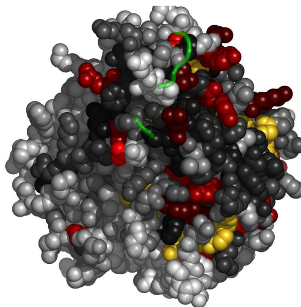
Fig. 5. Residues in 1a4gA, at the interface with 1a4gA1, colored by their relative importance. 1a4gA1 is shown in backbone representation (See Appendix for the coloring scheme for the protein chain 1a4gA.)
