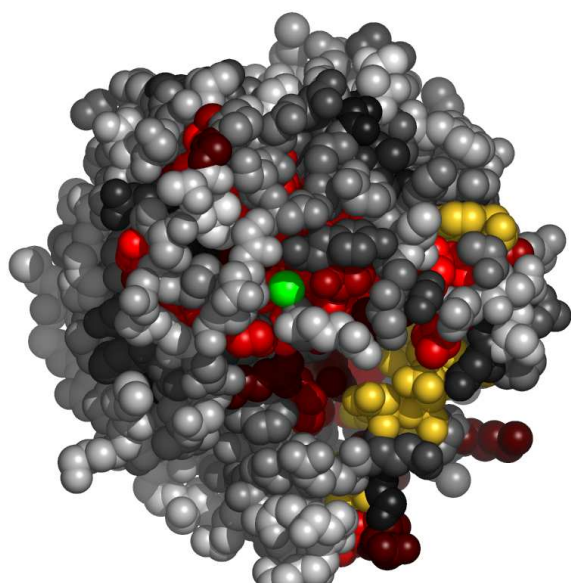
Fig. 7. Residues in 1a4gA, at the interface with calcium ion, colored by their relative importance. The ligand (calcium ion) is colored green. Atoms further than 30Å away from the geometric center of the ligand, as well as on the line of sight to the ligand were removed. (See Appendix for the coloring scheme for the protein chain 1a4gA.)
