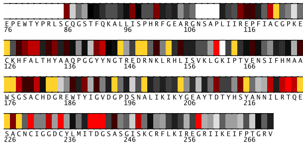
Fig. 1. Residues 76-270 in 1a4gA colored by their relative importance. (See Appendix, Fig.10, for the coloring scheme.)
