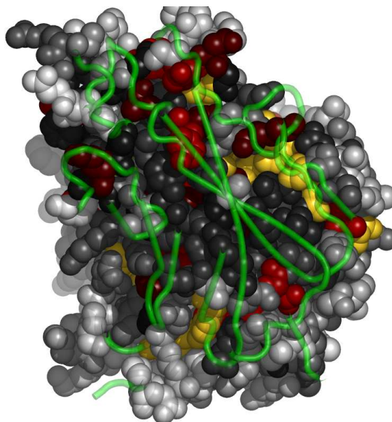
Fig. 9. Residues in 1a4gA, at the interface with 1a4gB, colored by their relative importance. 1a4gB is shown in backbone representation (See Appendix for the coloring scheme for the protein chain 1a4gA.)
