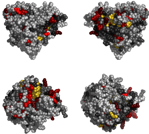
Fig. 3. Residues in 1a4gA, colored by their relative importance. Clockwise: front, back, top and bottom views.
