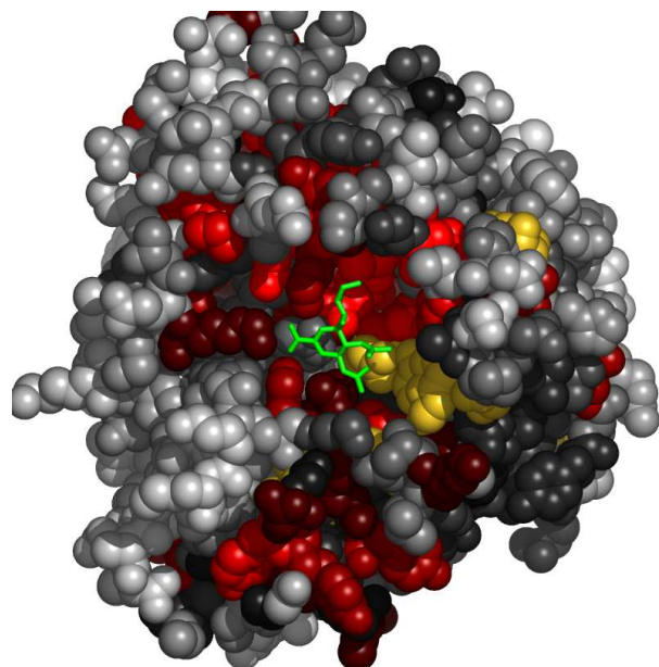
Fig. 8. Residues in 1a4gA, at the interface with zanamivir, colored by their relative importance. The ligand (zanamivir) is colored green. Atoms further than 30Å away from the geometric center of the ligand, as well as on the line of sight to the ligand were removed. (See Appendix for the coloring scheme for the protein chain 1a4gA.)
