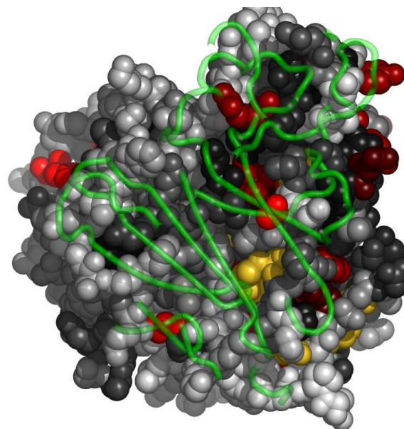
Fig. 6. Residues in 1a4gA, at the interface with 1a4gB1, colored by their relative importance. 1a4gB1 is shown in backbone representation (See Appendix for the coloring scheme for the protein chain 1a4gA.)
