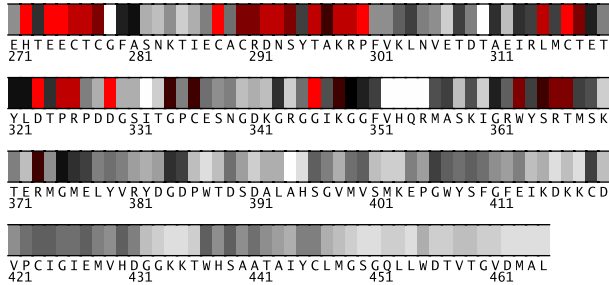
Fig. 2. Residues 271-465 in 1a4gA colored by their relative importance. (See Appendix, Fig.10, for the coloring scheme.)
