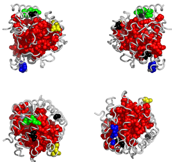
Fig. 4. Residues in 1a4mA, colored according to the cluster they belong to: red, followed by blue and yellow are the largest clusters (see Appendix for the coloring scheme). Clockwise: front, back, top and bottom views. The corresponding Pymol script is attached.
