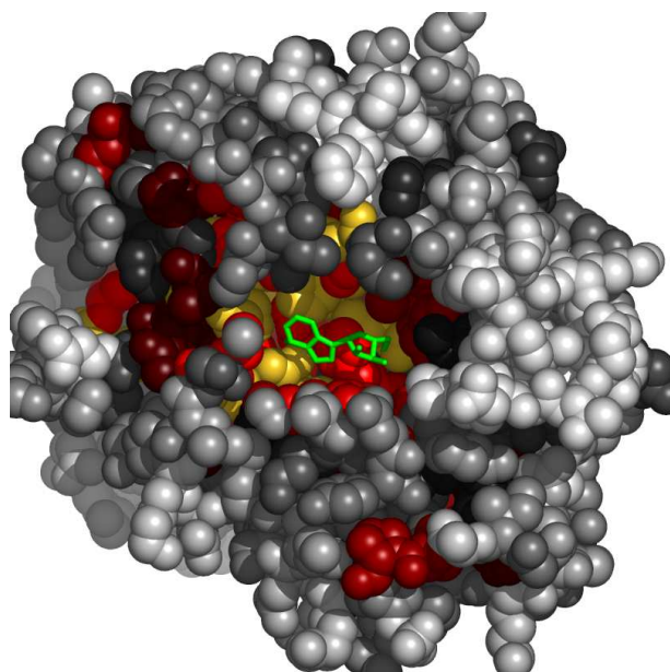
Fig. 5. Residues in 1a4mA, at the interface with PRH, colored by their relative importance. The ligand (PRH) is colored green. Atoms further than 30Å away from the geometric center of the ligand, as well as on the line of sight to the ligand were removed. (See Appendix for the coloring scheme for the protein chain 1a4mA.)
