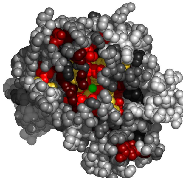
Fig. 6. Residues in 1a4mA, at the interface with zinc ion, colored by their relative importance. The ligand (zinc ion) is colored green. Atoms further than 30Å away from the geometric center of the ligand, as well as on the line of sight to the ligand were removed. (See Appendix for the coloring scheme for the protein chain 1a4mA.)
