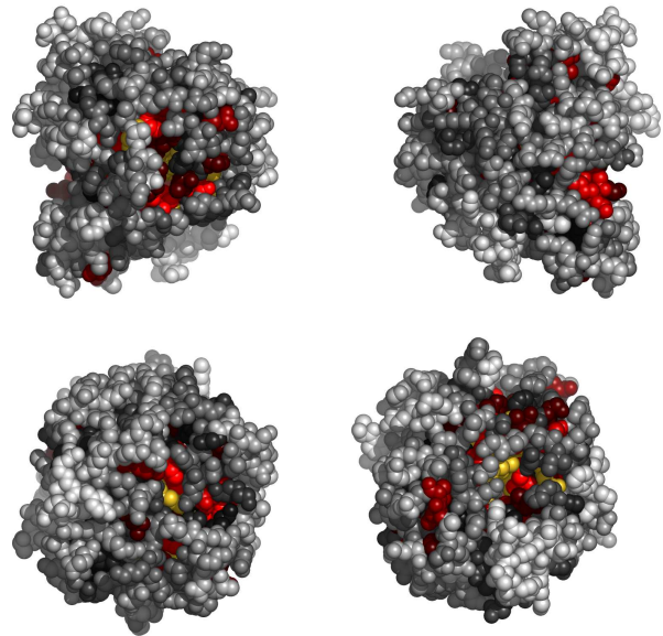
Fig. 3. Residues in 1a4mA, colored by their relative importance. Clockwise: front, back, top and bottom views.
