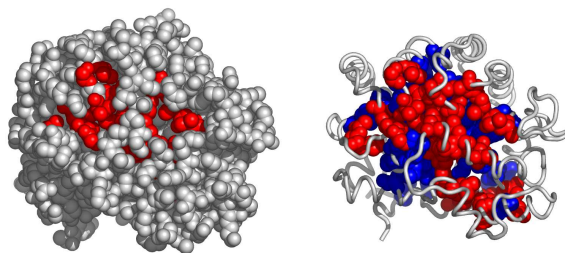
Fig. 8. A possible active surface on the chain 1a4mA. The larger cluster it belongs to is shown in blue.
