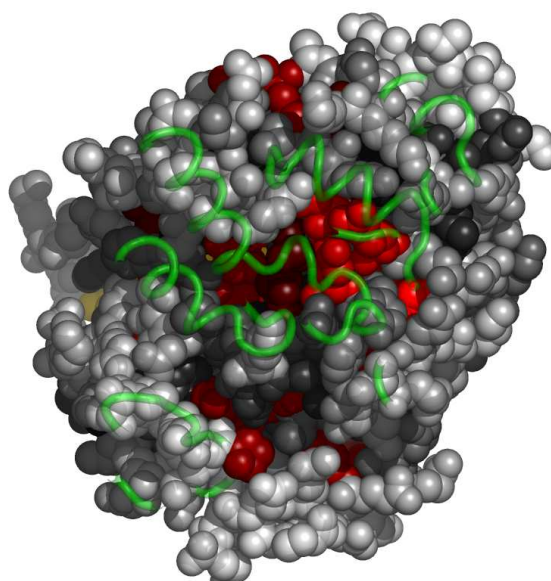
Fig. 7. Residues in 1a4mA, at the interface with 1a4mB, colored by their relative importance. 1a4mB is shown in backbone representation (See Appendix for the coloring scheme for the protein chain 1a4mA.)
