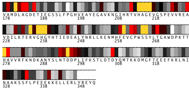
Fig. 2. Residues 178-352 in 1a4mA colored by their relative importance. (See Appendix, Fig.9, for the coloring scheme.)
