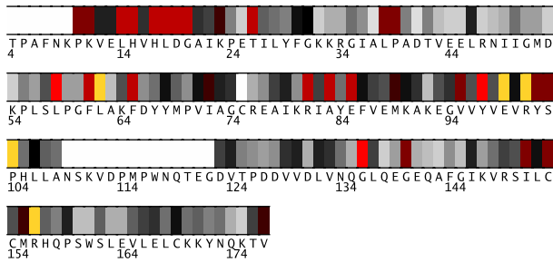
Fig. 1. Residues 4-177 in 1a4mA colored by their relative importance. (See Appendix, Fig.9, for the coloring scheme.)
