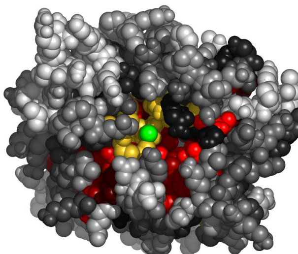
Fig. 5. Residues in 1a5iA, at the interface with methylene group, colored by their relative importance. The ligand (methylene group) is colored green. Atoms further than 30Å away from the geometric center of the ligand, as well as on the line of sight to the ligand were removed. (See Appendix for the coloring scheme for the protein chain 1a5iA.)
