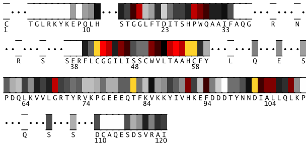
Fig. 1. Residues 1-121 in 1a5iA colored by their relative importance. (See Appendix, Fig.7, for the coloring scheme.) Note that some residues in 1a5iA carry insertion code.
