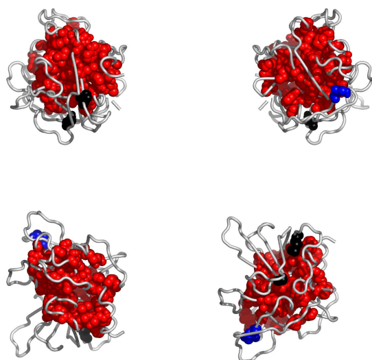
Fig. 4. Residues in 1a5iA, colored according to the cluster they belong to: red, followed by blue and yellow are the largest clusters (see Appendix for the coloring scheme). Clockwise: front, back, top and bottom views. The corresponding Pymol script is attached.
