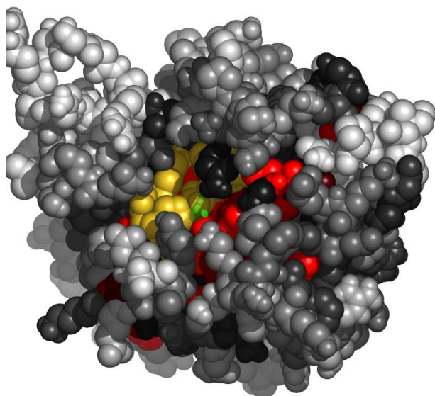
Fig. 6. Residues in 1a5iA, at the interface with 1a5iI, colored by their relative importance. 1a5iI is shown in backbone representation (See Appendix for the coloring scheme for the protein chain 1a5iA.)
