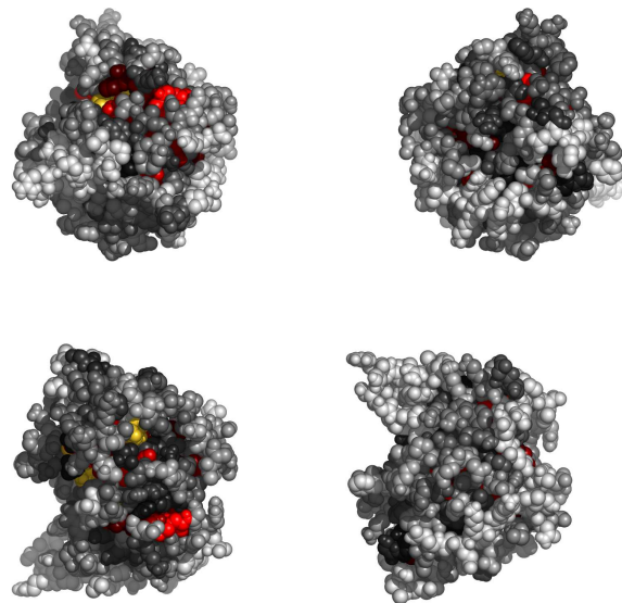
Fig. 3. Residues in 1a5iA, colored by their relative importance. Clockwise: front, back, top and bottom views.
