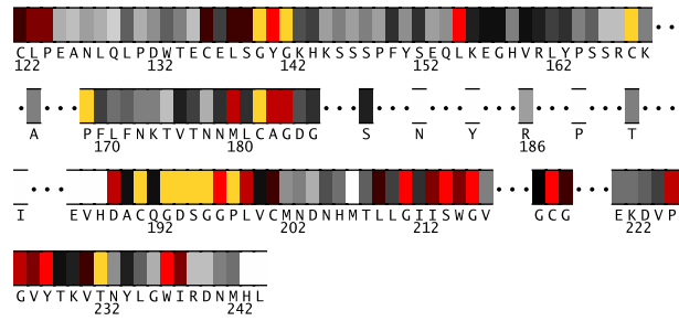
Fig. 2. Residues 122-244 in 1a5iA colored by their relative importance. (See Appendix, Fig.7, for the coloring scheme.) Note that some residues in 1a5iA carry insertion code.
