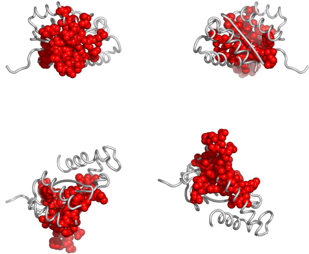
Fig. 3. Residues in 1a5xA, colored according to the cluster they belong to: red, followed by blue and yellow are the largest clusters (see Appendix for the coloring scheme). Clockwise: front, back, top and bottom views. The corresponding Pymol script is attached.
