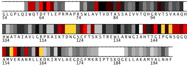
Fig. 1. Residues 54-199 in 1a5xA colored by their relative importance. (See Appendix, Fig.7, for the coloring scheme.)
