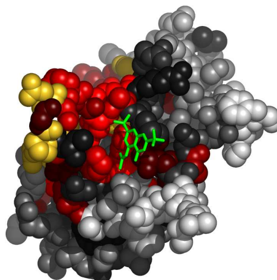
Fig. 5. Residues in 1a5xA, at the interface with Y3, colored by their relative importance. The ligand (Y3) is colored green. Atoms further than 30Å away from the geometric center of the ligand, as well as on the line of sight to the ligand were removed. (See Appendix for the coloring scheme for the protein chain 1a5xA.)
