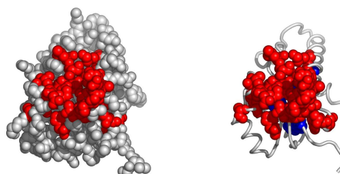
Fig. 6. A possible active surface on the chain 1a5xA. The larger cluster it belongs to is shown in blue.
