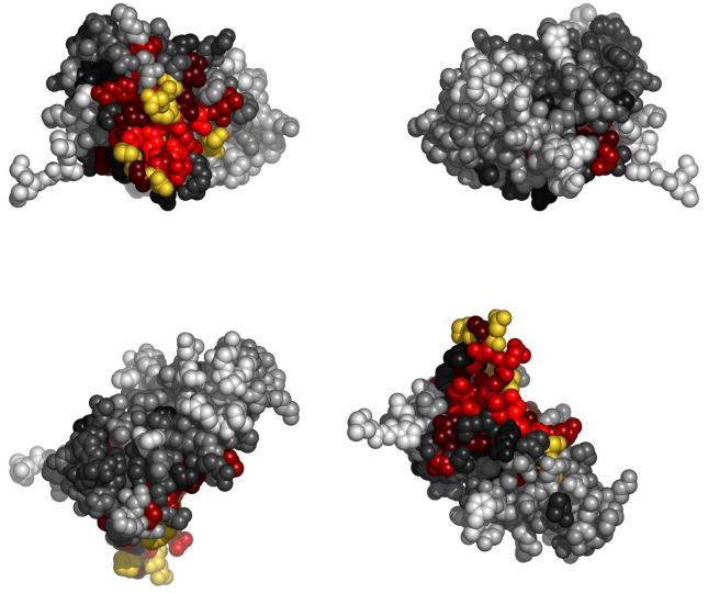
Fig. 2. Residues in 1a5xA, colored by their relative importance. Clockwise: front, back, top and bottom views.
