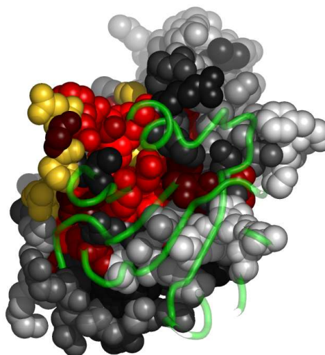
Fig. 4. Residues in 1a5xA, at the interface with 1a5xA1, colored by their relative importance. 1a5xA1 is shown in backbone representation (See Appendix for the coloring scheme for the protein chain 1a5xA.)
