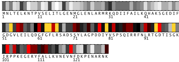
Fig. 1. Residues 1-130 in 1a63A colored by their relative importance. (See Appendix, Fig.5, for the coloring scheme.)
