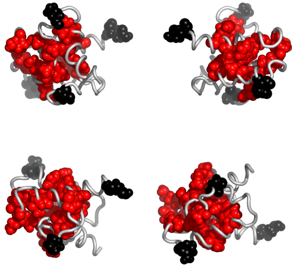
Fig. 3. Residues in 1a6sA, colored according to the cluster they belong to: red, followed by blue and yellow are the largest clusters (see Appendix for the coloring scheme). Clockwise: front, back, top and bottom views. The corresponding Pymol script is attached.
