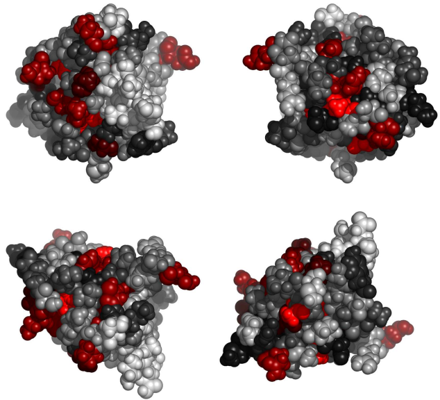
Fig. 2. Residues in 1a6sA, colored by their relative importance. Clockwise: front, back, top and bottom views.
