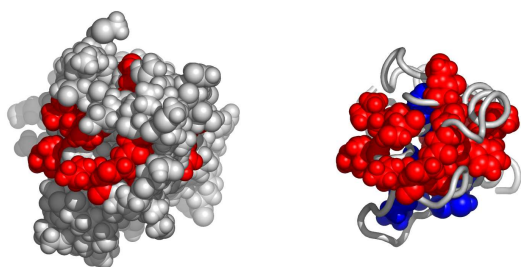
Fig. 4. A possible active surface on the chain 1a6sA. The larger cluster it belongs to is shown in blue.
