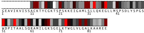
Fig. 1. Residues 1-87 in 1a6sA colored by their relative importance. (See Appendix, Fig.5, for the coloring scheme.)
