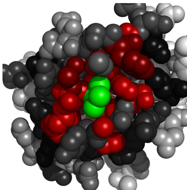
Fig. 4. Residues in 1a70A, at the interface with FES, colored by their relative importance. The ligand (FES) is colored green. Atoms further than 30Å away from the geometric center of the ligand, as well as on the line of sight to the ligand were removed. (See Appendix for the coloring scheme for the protein chain 1a70A.)
