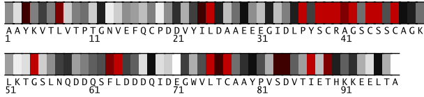
Fig. 1. Residues 1-97 in 1a70A colored by their relative importance. (See Appendix, Fig.6, for the coloring scheme.)
