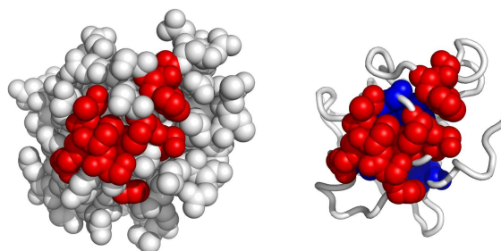
Fig. 5. A possible active surface on the chain 1a70A. The larger cluster it belongs to is shown in blue.
