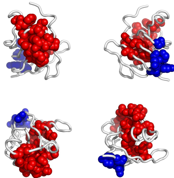
Fig. 3. Residues in 1a70A, colored according to the cluster they belong to: red, followed by blue and yellow are the largest clusters (see Appendix for the coloring scheme). Clockwise: front, back, top and bottom views. The corresponding Pymol script is attached.
