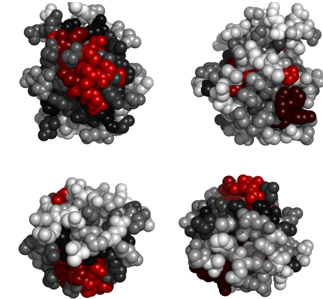
Fig. 1. Residues 1-97 in 1a70A colored by their relative importance. (See Appendix, Fig.6, for the coloring scheme.)
