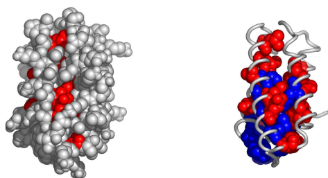
Fig. 5. A possible active surface on the chain 1a7eA. The larger cluster it belongs to is shown in blue.
