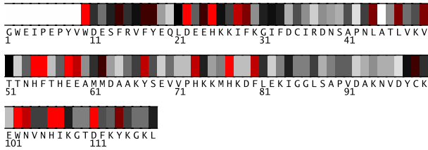
Fig. 1. Residues 1-118 in 1a7eA colored by their relative importance. (See Appendix, Fig.6, for the coloring scheme.)
