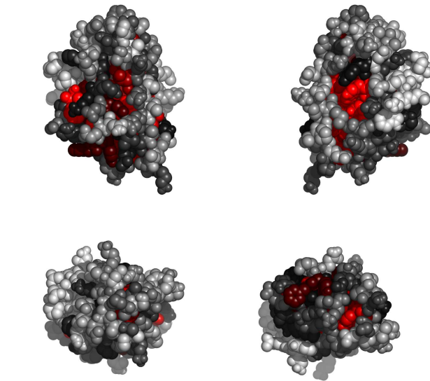
Fig. 1. Residues 1-118 in 1a7eA colored by their relative importance. (See Appendix, Fig.6, for the coloring scheme.)
