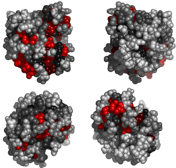
Fig. 2. Residues in 1a85A, colored by their relative importance. Clockwise: front, back, top and bottom views.
