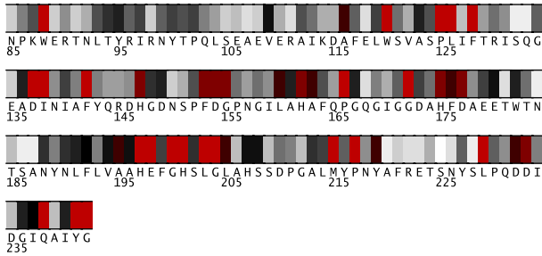
Fig. 1. Residues 85-242 in 1a85A colored by their relative importance. (See Appendix, Fig.12, for the coloring scheme.)
