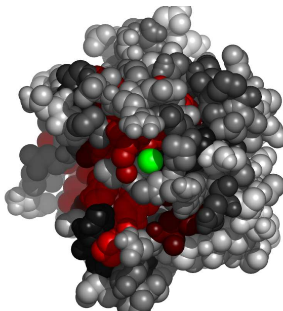
Fig. 6. Residues in 1a85A, at the interface with calcium ion, colored by their relative importance. The ligand (calcium ion) is colored green. Atoms further than 30Å away from the geometric center of the ligand, as well as on the line of sight to the ligand were removed. (See Appendix for the coloring scheme for the protein chain 1a85A.)
