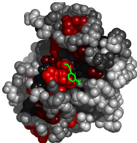
Fig. 5. Residues in 1a85A, at the interface with DBP, colored by their relative importance. The ligand (DBP) is colored green. Atoms further than 30Å away from the geometric center of the ligand, as well as on the line of sight to the ligand were removed. (See Appendix for the coloring scheme for the protein chain 1a85A.)
