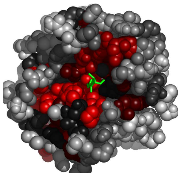
Fig. 8. Residues in 1a85A, at the interface with HMI, colored by their relative importance. The ligand (HMI) is colored green. Atoms further than 30\text{\AA} away from the geometric center of the ligand, as well as on the line of sight to the ligand were removed. (See Appendix for the coloring scheme for the protein chain 1a85A.)
