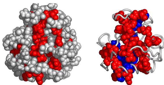
Fig. 11. A possible active surface on the chain 1a85A. The larger cluster it belongs to is shown in blue.
