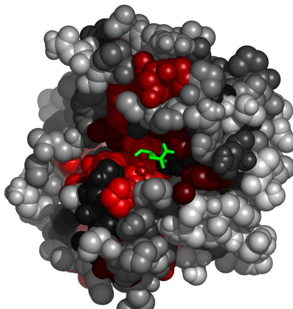
Fig. 9. Residues in 1a85A, at the interface with d-asparagine, colored by their relative importance. The ligand (d-asparagine) is colored green. Atoms further than 30\text{\AA} away from the geometric center of the ligand, as well as on the line of sight to the ligand were removed. (See Appendix for the coloring scheme for the protein chain 1a85A.)
