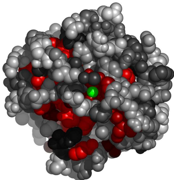
Fig. 10. Residues in 1a85A, at the interface with zinc ion, colored by their relative importance. The ligand (zinc ion) is colored green. Atoms further than 30Å away from the geometric center of the ligand, as well as on the line of sight to the ligand were removed. (See Appendix for the coloring scheme for the protein chain 1a85A.)
