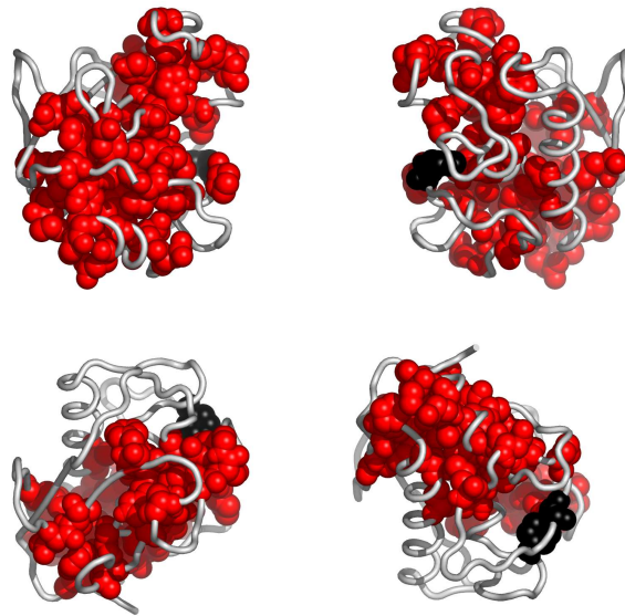
Fig. 3. Residues in 1a85A, colored according to the cluster they belong to: red, followed by blue and yellow are the largest clusters (see Appendix for the coloring scheme). Clockwise: front, back, top and bottom views. The corresponding Pymol script is attached.
