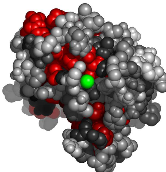
Fig. 4. Residues in 1a85A, at the interface with calcium ion, colored by their relative importance. The ligand (calcium ion) is colored green. Atoms further than 30Å away from the geometric center of the ligand, as well as on the line of sight to the ligand were removed. (See Appendix for the coloring scheme for the protein chain 1a85A.)
