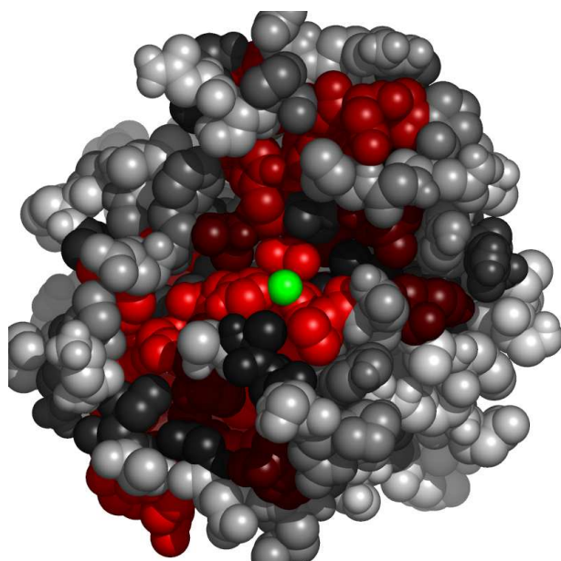
Fig. 7. Residues in 1a85A, at the interface with zinc ion, colored by their relative importance. The ligand (zinc ion) is colored green. Atoms further than 30Å away from the geometric center of the ligand, as well as on the line of sight to the ligand were removed. (See Appendix for the coloring scheme for the protein chain 1a85A.)
