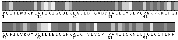
Fig. 1. Residues 1-99 in 1a9mA colored by their relative importance. (See Appendix, Fig.4, for the coloring scheme.)
