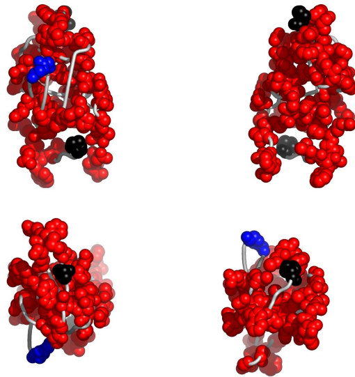
Fig. 3. Residues in 1a9mA, colored according to the cluster they belong to: red, followed by blue and yellow are the largest clusters (see Appendix for the coloring scheme). Clockwise: front, back, top and bottom views. The corresponding Pymol script is attached.
