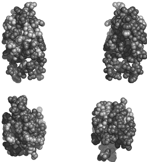
Fig. 2. Residues in 1a9mA, colored by their relative importance. Clockwise: front, back, top and bottom views.
