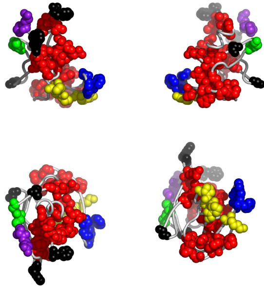
Fig. 3. Residues in IaaqA, colored according to the cluster they belong to: red, followed by blue and yellow are the largest clusters (see Appendix for the coloring scheme). Clockwise: front, back, top and bottom views. The corresponding Pymol script is attached.
