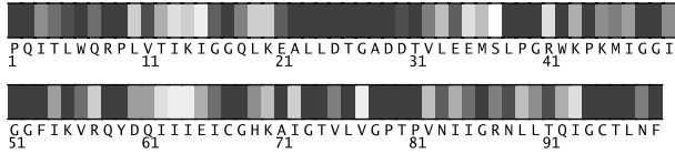
Fig. 1. Residues 1-99 in IaaqA colored by their relative importance. (See Appendix, Fig.4, for the coloring scheme.)
