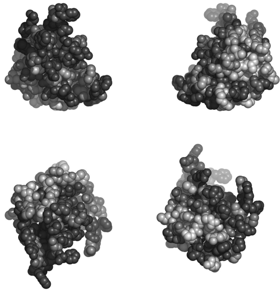
Fig. 2. Residues in IaaqA, colored by their relative importance. Clockwise: front, back, top and bottom views.
