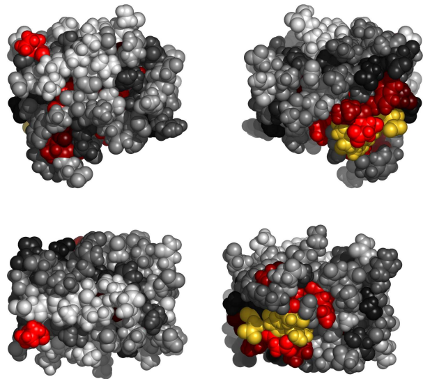
Fig. 2. Residues in lab7A, colored by their relative importance. Clockwise: front, back, top and bottom views.
