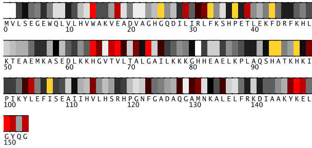
Fig. 1. Residues 0-153 in IabsA colored by their relative importance. (See Appendix, Fig.7, for the coloring scheme.)
