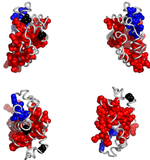
Fig. 3. Residues in IabsA, colored according to the cluster they belong to: red, followed by blue and yellow are the largest clusters (see Appendix for the coloring scheme). Clockwise: front, back, top and bottom views. The corresponding Pymol script is attached.
