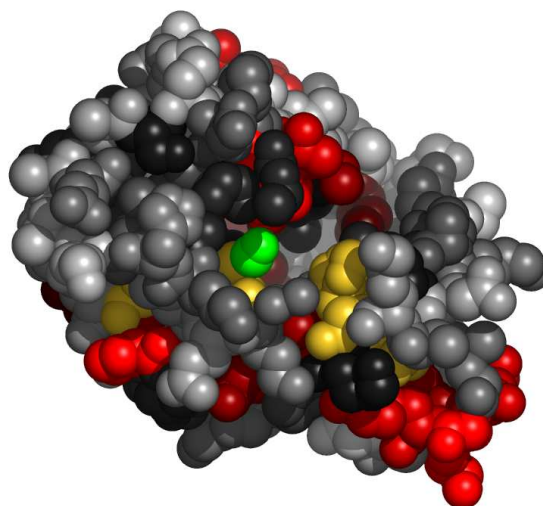
Fig. 4. Residues in labsA, at the interface with carbon monoxide, colored by their relative importance. The ligand (carbon monoxide) is colored green. Atoms further than 30Å away from the geometric center of the ligand, as well as on the line of sight to the ligand were removed. (See Appendix for the coloring scheme for the protein chain labsA.)
