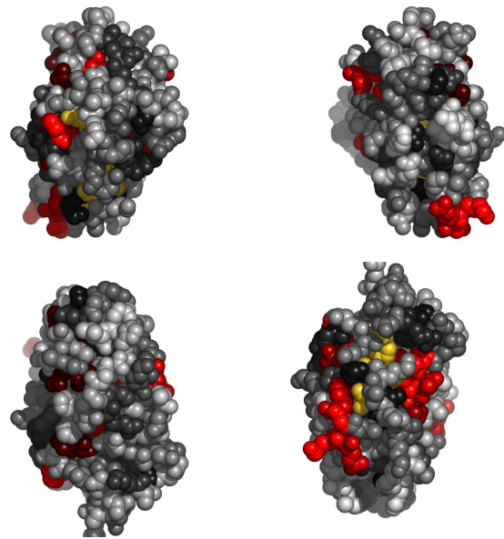
Fig. 2. Residues in IabsA, colored by their relative importance. Clockwise: front, back, top and bottom views.
