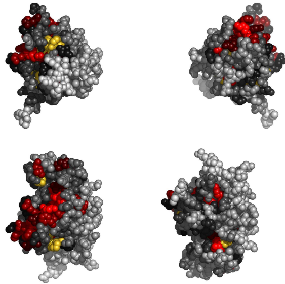
Fig. 2. Residues in Iad6A, colored by their relative importance. Clockwise: front, back, top and bottom views.
