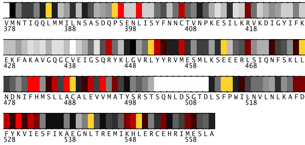
Fig. 1. Residues 378-562 in Iad6A colored by their relative importance. (See Appendix, Fig.5, for the coloring scheme.)
