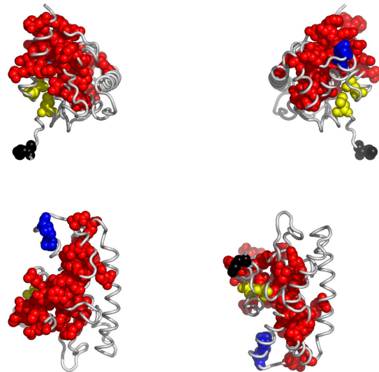
Fig. 3. Residues in Iad6A, colored according to the cluster they belong to: red, followed by blue and yellow are the largest clusters (see Appendix for the coloring scheme). Clockwise: front, back, top and bottom views. The corresponding Pymol script is attached.
