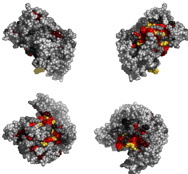
Fig. 3. Residues in IadiA, colored by their relative importance. Clockwise: front, back, top and bottom views.
