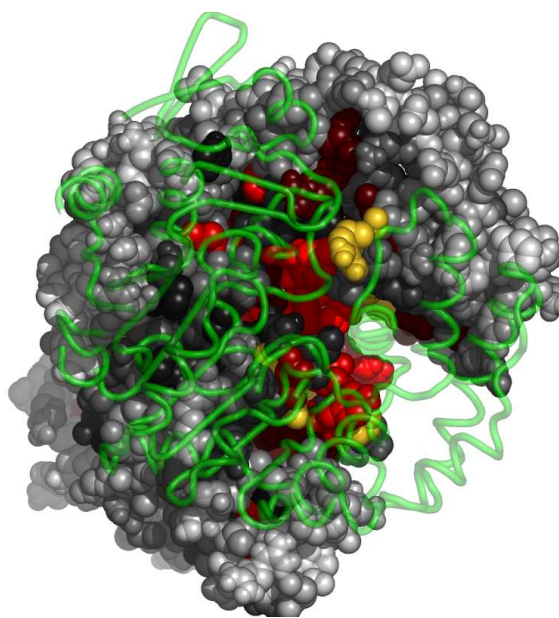
Fig. 5. Residues in IadiA, at the interface with IadiB, colored by their relative importance. IadiB is shown in backbone representation (See Appendix for the coloring scheme for the protein chain IadiA.)
