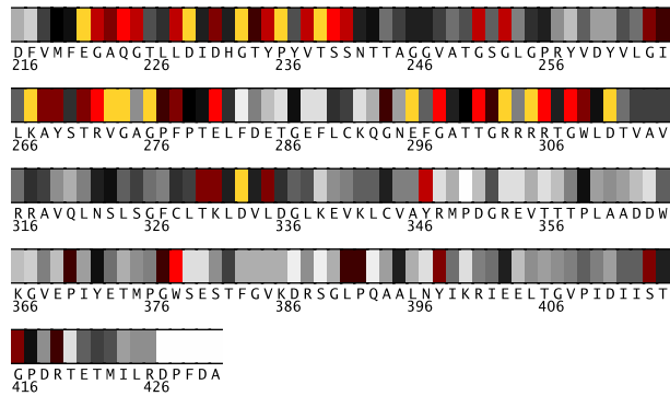
Fig. 2. Residues 216-431 in IadiA colored by their relative importance. (See Appendix, Fig.7, for the coloring scheme.)
