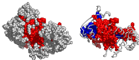
Fig. 6. A possible active surface on the chain IadiA. The larger cluster it belongs to is shown in blue.
