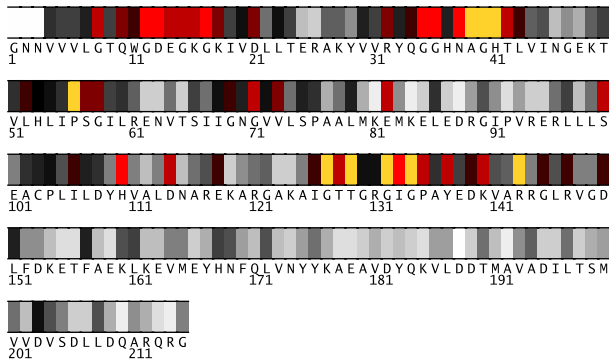
Fig. 1. Residues 1-215 in IadiA colored by their relative importance. (See Appendix, Fig.7, for the coloring scheme.)
