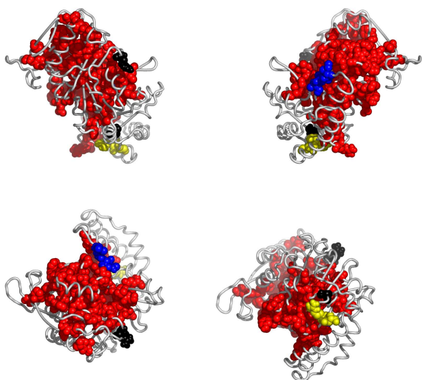
Fig. 4. Residues in 1adiA, colored according to the cluster they belong to: red, followed by blue and yellow are the largest clusters (see Appendix for the coloring scheme). Clockwise: front, back, top and bottom views. The corresponding Pymol script is attached.
