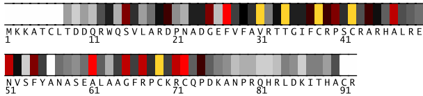
Fig. 1. Residues 1-92 in IadnA colored by their relative importance. (See Appendix, Fig.6, for the coloring scheme.)
