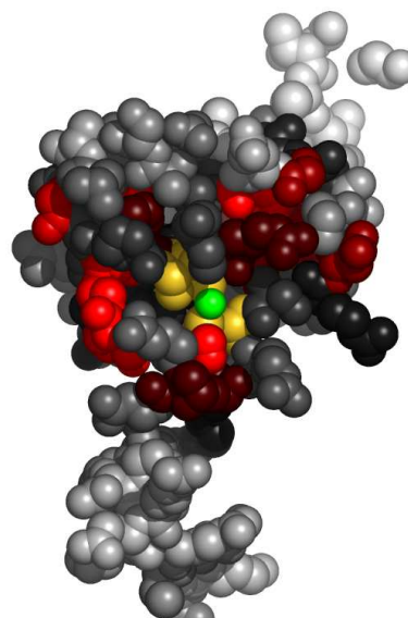
Fig. 4. Residues in ladnA, at the interface with zinc ion, colored by their relative importance. The ligand (zinc ion) is colored green. Atoms further than 30Å away from the geometric center of the ligand, as well as on the line of sight to the ligand were removed. (See Appendix for the coloring scheme for the protein chain ladnA.)
