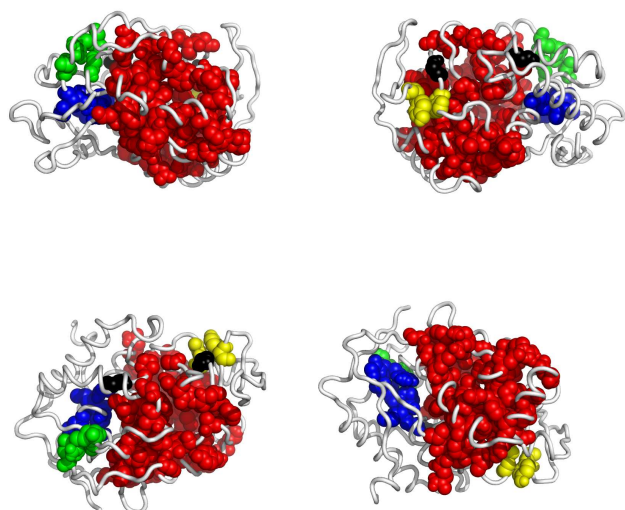
Fig. 4. Residues in IaesA, colored according to the cluster they belong to: red, followed by blue and yellow are the largest clusters (see Appendix for the coloring scheme). Clockwise: front, back, top and bottom views. The corresponding Pymol script is attached.
