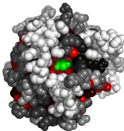
Fig. 5. Residues in IaesA, at the interface with imidazole, colored by their relative importance. The ligand (imidazole) is colored green. Atoms further than 30 Å away from the geometric center of the ligand, as well as on the line of sight to the ligand were removed. (See Appendix for the coloring scheme for the protein chain IaesA.)
