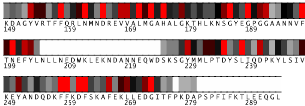
Fig. 2. Residues 149-294 in laesA colored by their relative importance. (See Appendix, Fig.8, for the coloring scheme.)
