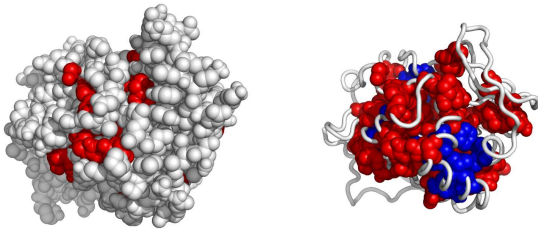
Fig. 7. A possible active surface on the chain laesaA. The larger cluster it belongs to is shown in blue.
