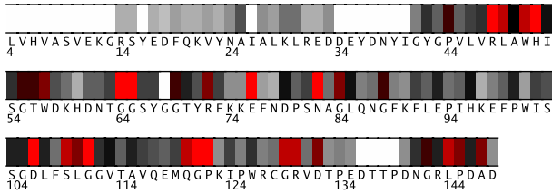
Fig. 1. Residues 4-148 in laesA colored by their relative importance. (See Appendix, Fig.8, for the coloring scheme.)
