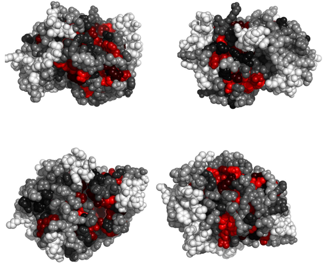
Fig. 2. Residues 149-294 in laesA colored by their relative importance. (See Appendix, Fig.8, for the coloring scheme.)
