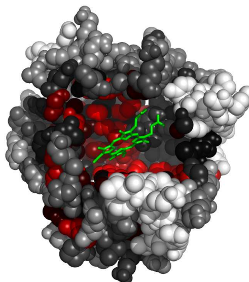
Fig. 6. Residues in laesA, at the interface with HEM, colored by their relative importance. The ligand (HEM) is colored green. Atoms further than 30Å away from the geometric center of the ligand, as well as on the line of sight to the ligand were removed. (See Appendix for the coloring scheme for the protein chain laesA.)
