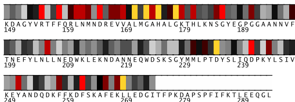
Fig. 2. Residues 149-294 in laetA colored by their relative importance. (See Appendix, Fig.9, for the coloring scheme.)
