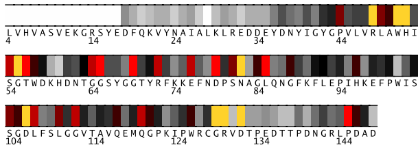
Fig. 1. Residues 4-148 in laetA colored by their relative importance. (See Appendix, Fig.9, for the coloring scheme.)
