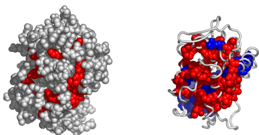
Fig. 6. Residues in laetA, at the interface with HEM, colored by their relative importance. The ligand (HEM) is colored green. Atoms further than 30Å away from the geometric center of the ligand, as well as on the line of sight to the ligand were removed. (See Appendix for the coloring scheme for the protein chain laetA.)
