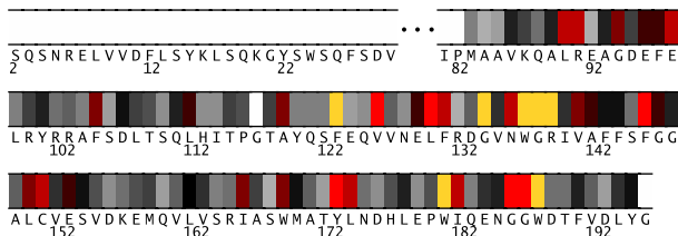
Fig. 1. Residues 2-196 in 1af3A colored by their relative importance. (See Appendix, Fig.5, for the coloring scheme.)
