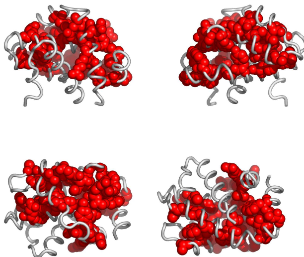
Fig. 1. Residues 2-196 in 1af3A colored by their relative importance. (See Appendix, Fig.5, for the coloring scheme.)
