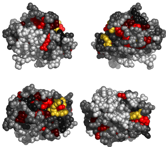
Fig. 2. Residues in 1af3A, colored by their relative importance. Clockwise: front, back, top and bottom views.
