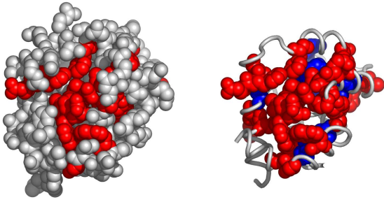
Fig. 4. A possible active surface on the chain 1af3A. The larger cluster it belongs to is shown in blue.
