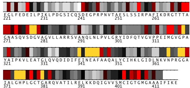
Fig. 2. Residues 221-417 in 1afwB colored by their relative importance. (See Appendix, Fig.9, for the coloring scheme.)
