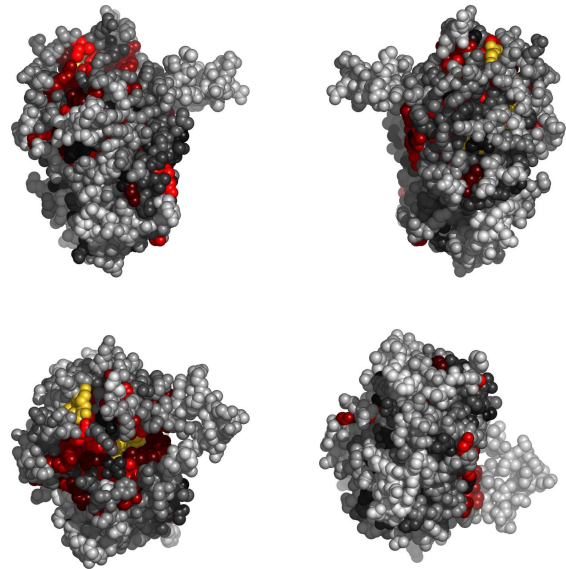
Fig. 2. Residues 221-417 in 1afwB colored by their relative importance. (See Appendix, Fig.9, for the coloring scheme.)
