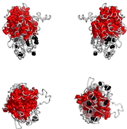
Fig. 4. Residues in 1afwB, colored according to the cluster they belong to: red, followed by blue and yellow are the largest clusters (see Appendix for the coloring scheme). Clockwise: front, back, top and bottom views. The corresponding Pymol script is attached.
