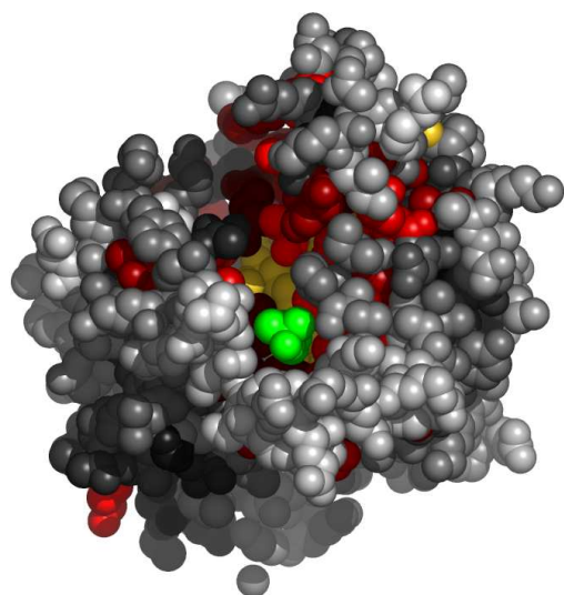
Fig. 6. Residues in 1afwB, at the interface with MRD, colored by their relative importance. The ligand (MRD) is colored green. Atoms further than 30Å away from the geometric center of the ligand, as well as on the line of sight to the ligand were removed. (See Appendix for the coloring scheme for the protein chain 1afwB.)
