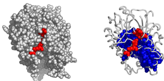
Fig. 7. A possible active surface on the chain 1afwB. The larger cluster it belongs to is shown in blue.
