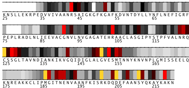
Fig. 1. Residues 25-220 in 1afwB colored by their relative importance. (See Appendix, Fig.9, for the coloring scheme.)
