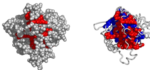
Fig. 8. Another possible active surface on the chain 1afwB. The larger cluster it belongs to is shown in blue.
