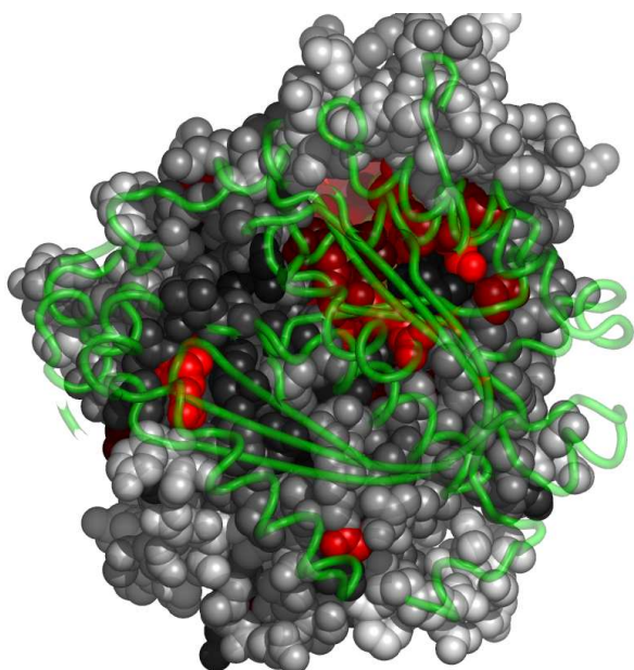
Fig. 5. Residues in 1afwB, at the interface with 1afwA, colored by their relative importance. 1afwA is shown in backbone representation (See Appendix for the coloring scheme for the protein chain 1afwB.)
