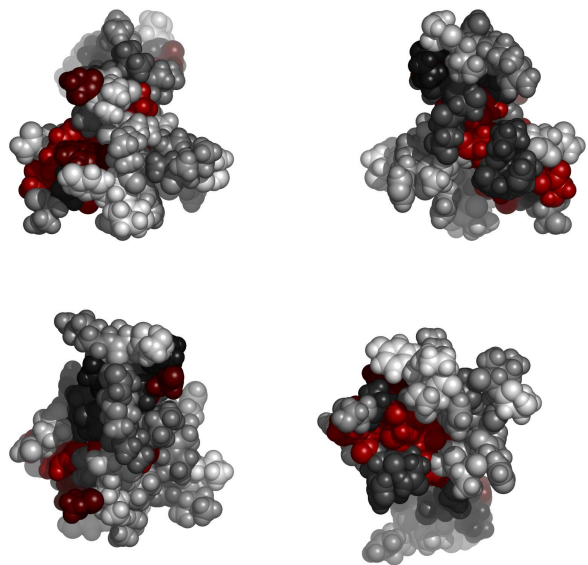
Fig. 2. Residues in 1ahlA, colored by their relative importance. Clockwise: front, back, top and bottom views.
