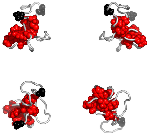
Fig. 3. Residues in 1ahlA, colored according to the cluster they belong to: red, followed by blue and yellow are the largest clusters (see Appendix for the coloring scheme). Clockwise: front, back, top and bottom views. The corresponding Pymol script is attached.
