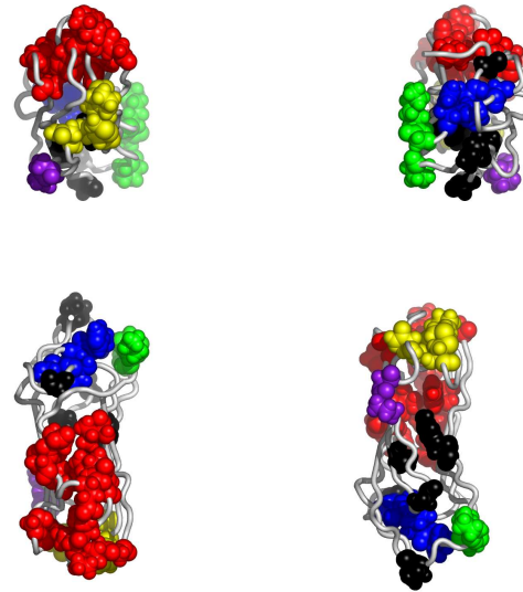
Fig. 3. Residues in lahmA, colored according to the cluster they belong to: red, followed by blue and yellow are the largest clusters (see Appendix for the coloring scheme). Clockwise: front, back, top and bottom views. The corresponding Pymol script is attached.
