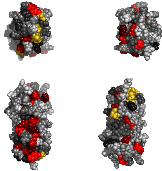
Fig. 2. Residues in lahmA, colored by their relative importance. Clockwise: front, back, top and bottom views.
