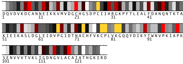
Fig. 1. Residues 1-129 in lahmA colored by their relative importance. (See Appendix, Fig.5, for the coloring scheme.)
