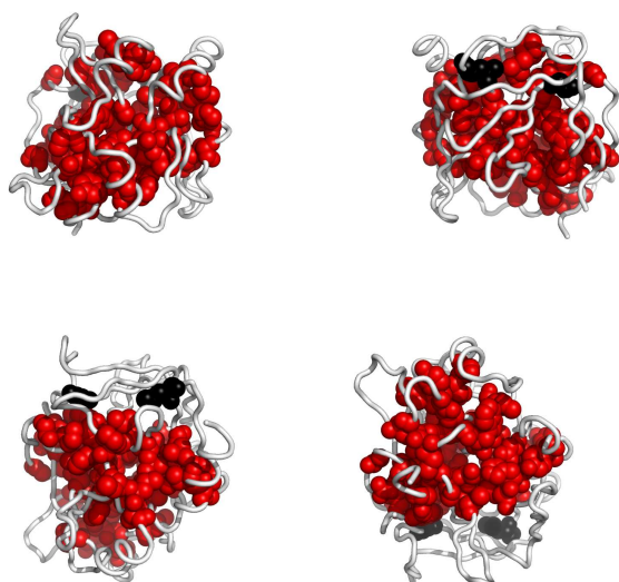
Fig. 4. Residues in 1ahtH, colored according to the cluster they belong to: red, followed by blue and yellow are the largest clusters (see Appendix for the coloring scheme). Clockwise: front, back, top and bottom views. The corresponding Pymol script is attached.
