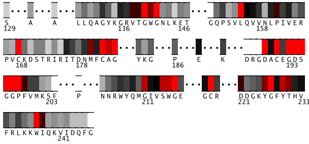
Fig. 2. Residues 129-246 in 1ahtH colored by their relative importance. (See Appendix, Fig.8, for the coloring scheme.) Note that some residues in 1ahtH carry insertion code.
