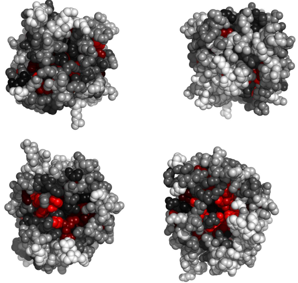
Fig. 3. Residues in 1ahtH, colored by their relative importance. Clockwise: front, back, top and bottom views.
