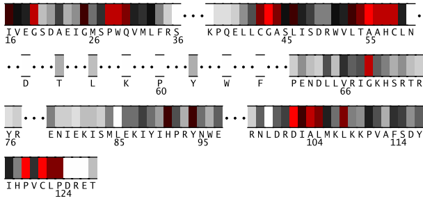
Fig. 1. Residues 16-128 in 1ahtH colored by their relative importance. (See Appendix, Fig.8, for the coloring scheme.) Note that some residues in 1ahtH carry insertion code.
