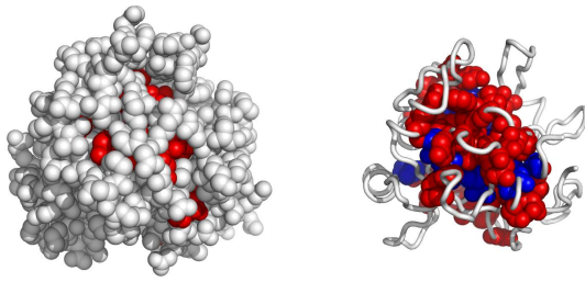
Fig. 7. A possible active surface on the chain lahtH. The larger cluster it belongs to is shown in blue.
