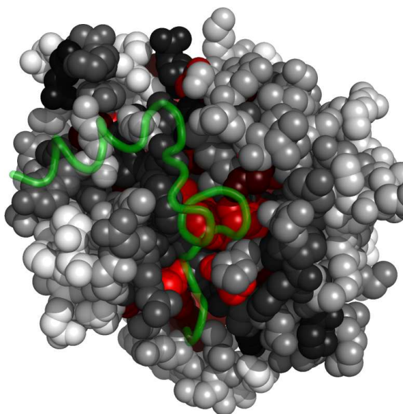
Fig. 6. Residues in 1ahtH, at the interface with 1ahtL, colored by their relative importance. 1ahtL is shown in backbone representation (See Appendix for the coloring scheme for the protein chain 1ahtH.)
