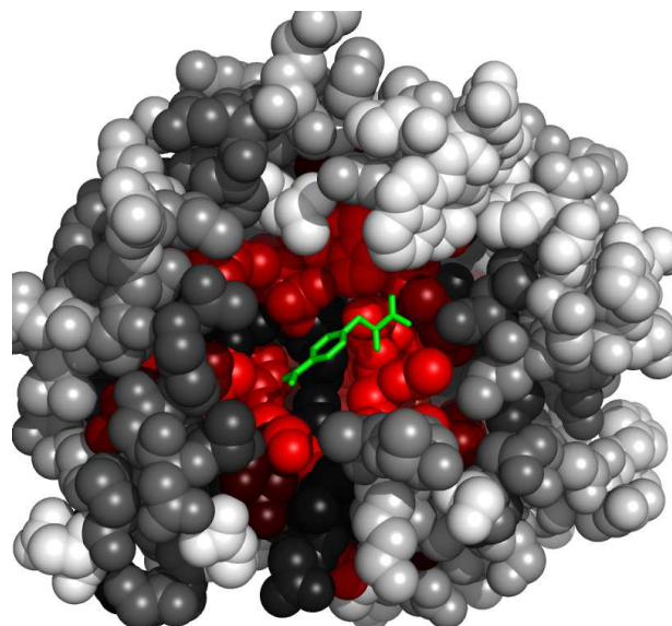
Fig. 5. Residues in 1ahtH, at the interface with APA, colored by their relative importance. The ligand (APA) is colored green. Atoms further than 30 Å away from the geometric center of the ligand, as well as on the line of sight to the ligand were removed. (See Appendix for the coloring scheme for the protein chain 1ahtH.)
