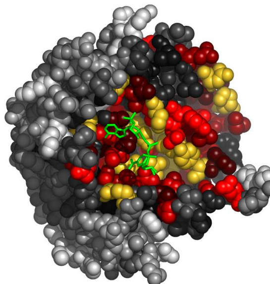
Fig. 5. Residues in lai3A, at the interface with NDO, colored by their relative importance. The ligand (NDO) is colored green. Atoms further than 30Å away from the geometric center of the ligand, as well as on the line of sight to the ligand were removed. (See Appendix for the coloring scheme for the protein chain lai3A.)
