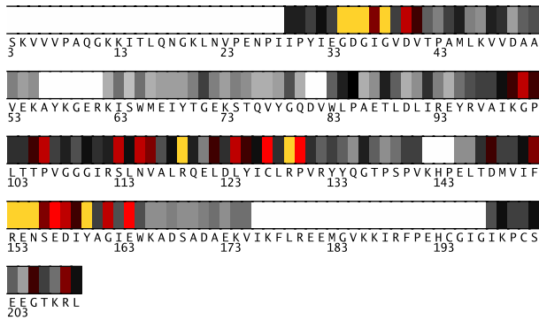
Fig. 1. Residues 3-209 in 1ai3A colored by their relative importance. (See Appendix, Fig.8, for the coloring scheme.)
