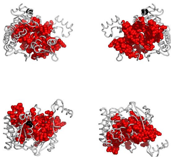
Fig. 4. Residues in 1ai3A, colored according to the cluster they belong to: red, followed by blue and yellow are the largest clusters (see Appendix for the coloring scheme). Clockwise: front, back, top and bottom views. The corresponding Pymol script is attached.
