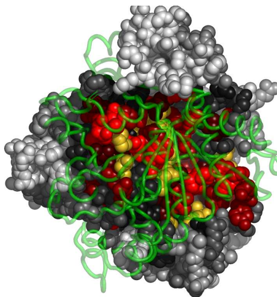
Fig. 6. Residues in 1ai3A, at the interface with 1ai3A1, colored by their relative importance. 1ai3A1 is shown in backbone representation (See Appendix for the coloring scheme for the protein chain 1ai3A.)
