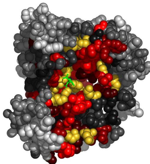
Fig. 7. Residues in 1ai3A, at the interface with ITM, colored by their relative importance. The ligand (ITM) is colored green. Atoms further than 30Å away from the geometric center of the ligand, as well as on the line of sight to the ligand were removed. (See Appendix for the coloring scheme for the protein chain 1ai3A.)
