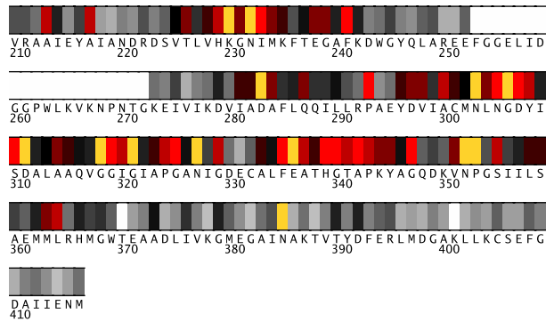
Fig. 2. Residues 210-416 in 1ai3A colored by their relative importance. (See Appendix, Fig.8, for the coloring scheme.)
