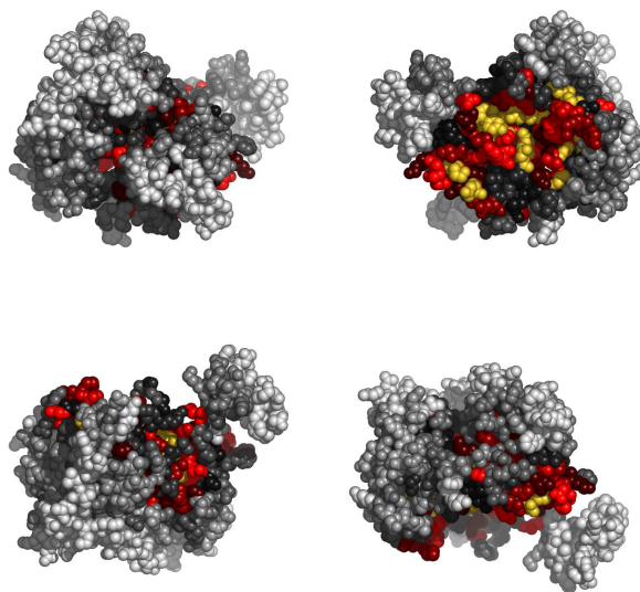
Fig. 3. Residues in 1ai3A, colored by their relative importance. Clockwise: front, back, top and bottom views.
