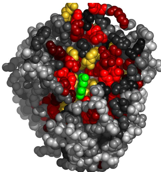
Fig. 9. Residues in 1aibA, at the interface with 2-oxyglutaric acid, colored by their relative importance. The ligand (2-oxyglutaric acid) is colored green. Atoms further than 30Å away from the geometric center of the ligand, as well as on the line of sight to the ligand were removed. (See Appendix for the coloring scheme for the protein chain 1aibA.)
