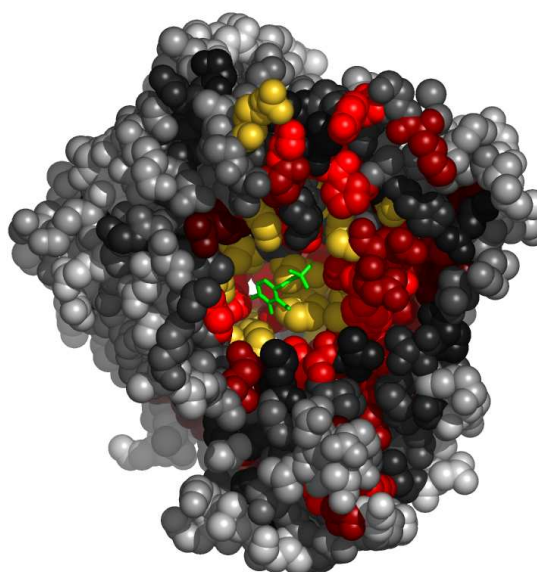
Fig. 7. Residues in 1aibA, at the interface with PMP, colored by their relative importance. The ligand (PMP) is colored green. Atoms further than 30Å away from the geometric center of the ligand, as well as on the line of sight to the ligand were removed. (See Appendix for the coloring scheme for the protein chain 1aibA.)
