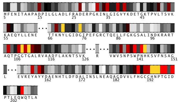
Fig. 1. Residues 5-209 in 1aibA colored by their relative importance. (See Appendix, Fig.10, for the coloring scheme.)
