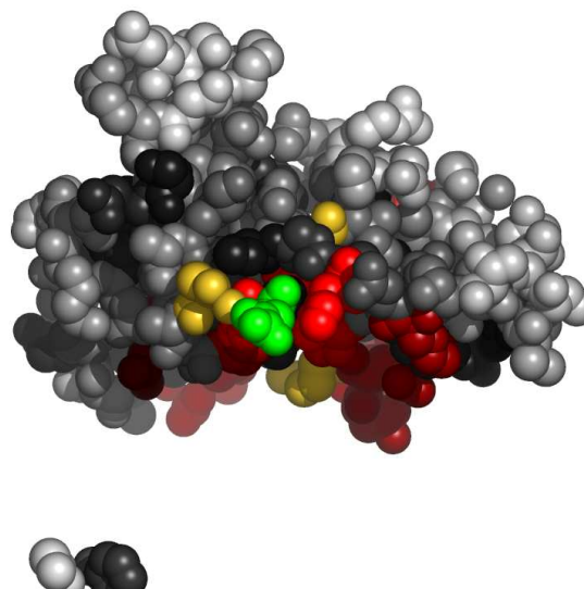
Fig. 6. Residues in 1aibA, at the interface with 2-oxyglutaric acid, colored by their relative importance. The ligand (2-oxyglutaric acid) is colored green. Atoms further than 30Å away from the geometric center of the ligand, as well as on the line of sight to the ligand were removed. (See Appendix for the coloring scheme for the protein chain 1aibA.)
