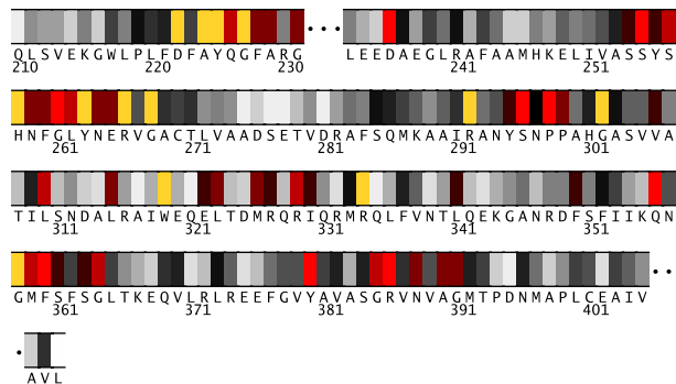
Fig. 2. Residues 210-409 in 1aibA colored by their relative importance. (See Appendix, Fig.10, for the coloring scheme.)
