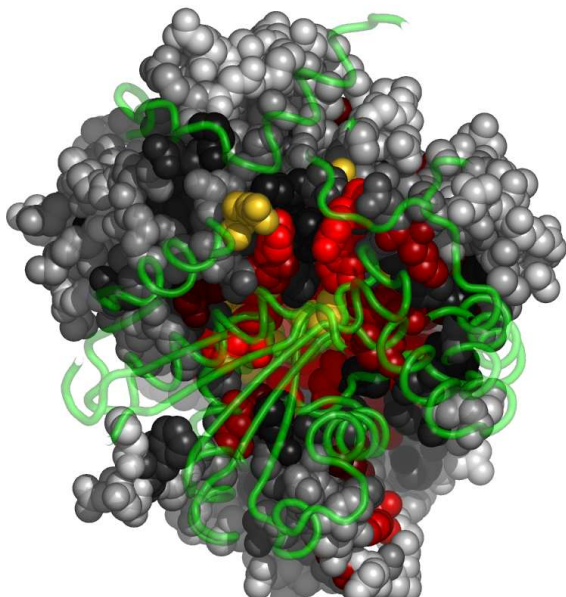
Fig. 8. Residues in 1aibA, at the interface with 1aibB, colored by their relative importance. 1aibB is shown in backbone representation (See Appendix for the coloring scheme for the protein chain 1aibA.)
