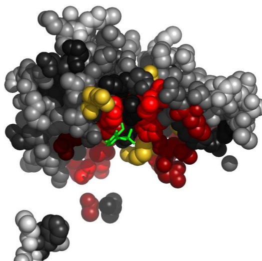
Fig. 5. Residues in 1aibA, at the interface with PMP, colored by their relative importance. The ligand (PMP) is colored green. Atoms further than 30Å away from the geometric center of the ligand, as well as on the line of sight to the ligand were removed. (See Appendix for the coloring scheme for the protein chain 1aibA.)
