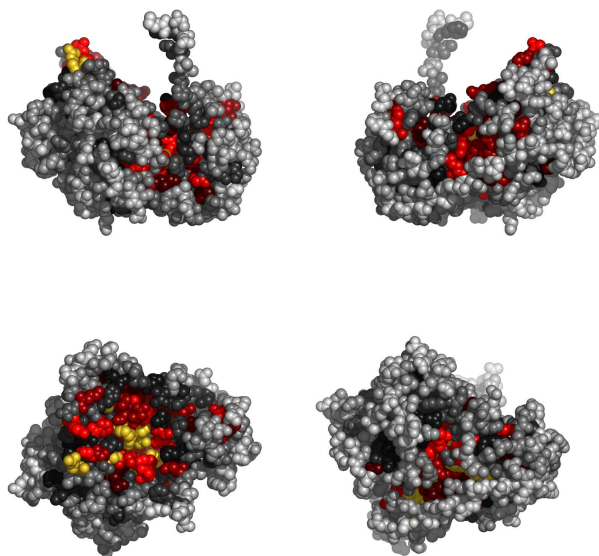
Fig. 2. Residues 210-409 in 1aibA colored by their relative importance. (See Appendix, Fig.10, for the coloring scheme.)
