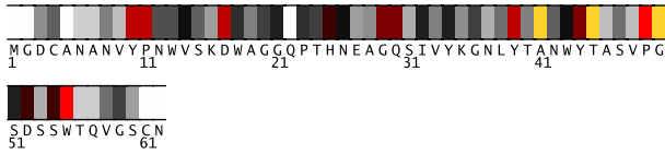
Fig. 1. Residues 1-62 in laiWA colored by their relative importance. (See Appendix, Fig.5, for the coloring scheme.)
