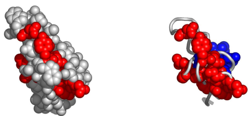
Fig. 4. A possible active surface on the chain laiWA. The larger cluster it belongs to is shown in blue.
