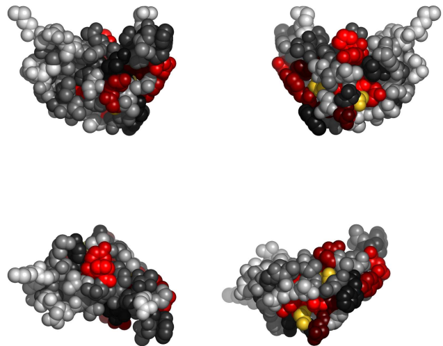
Fig. 1. Residues 1-62 in laiWA colored by their relative importance. (See Appendix, Fig.5, for the coloring scheme.)
