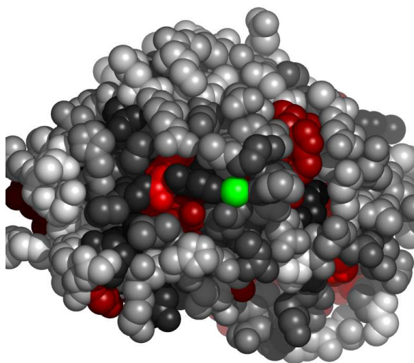
Fig. 5. Residues in IamyA, at the interface with calcium ion, colored by their relative importance. The ligand (calcium ion) is colored green. Atoms further than 30 Å away from the geometric center of the ligand, as well as on the line of sight to the ligand were removed. (See Appendix for the coloring scheme for the protein chain IamyA.)
