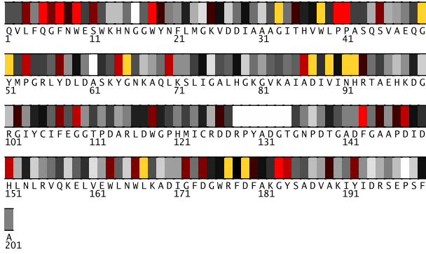
Fig. 1. Residues 1-201 in IamyA colored by their relative importance. (See Appendix, Fig.9, for the coloring scheme.)
