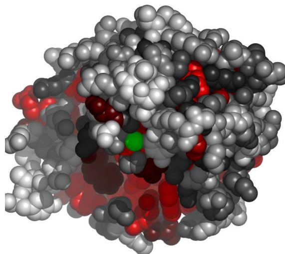
Fig. 7. Residues in 1amyA, at the interface with calcium ion, colored by their relative importance. The ligand (calcium ion) is colored green. Atoms further than 30Å away from the geometric center of the ligand, as well as on the line of sight to the ligand were removed. (See Appendix for the coloring scheme for the protein chain 1amyA.)
