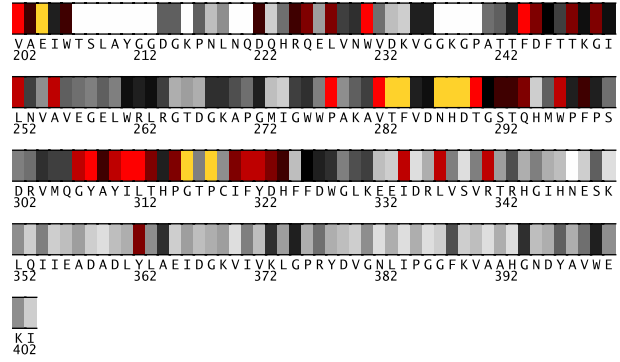
Fig. 2. Residues 202-403 in IamyA colored by their relative importance. (See Appendix, Fig.9, for the coloring scheme.)
