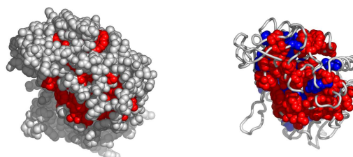
Fig. 8. A possible active surface on the chain 1amyA. The larger cluster it belongs to is shown in blue.
