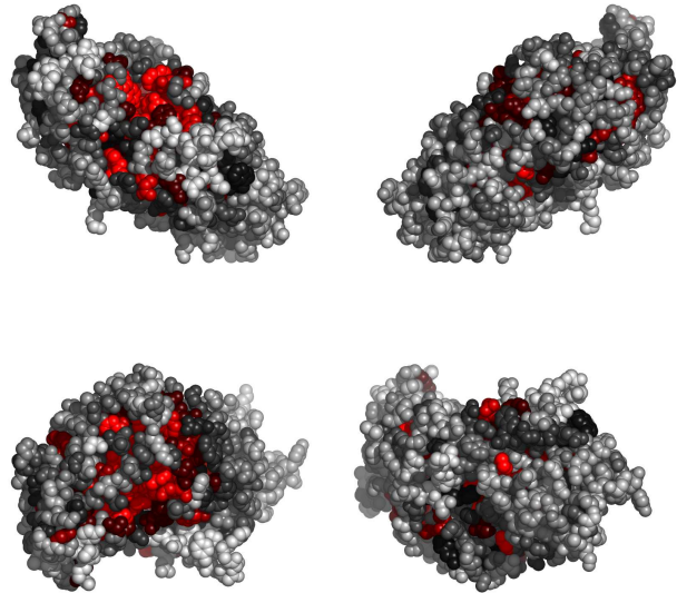
Fig. 3. Residues in IamyA, colored by their relative importance. Clockwise: front, back, top and bottom views.
