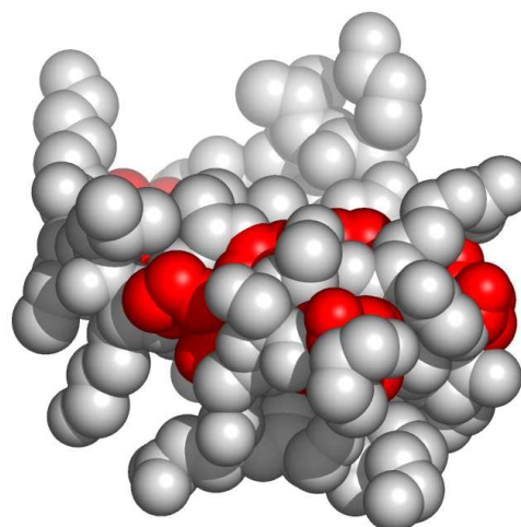
Fig. 4. Residues in 1an1I, at the interface with 1an1E, colored by their relative importance. 1an1E is shown in backbone representation (See Appendix for the coloring scheme for the protein chain 1an1I.)
