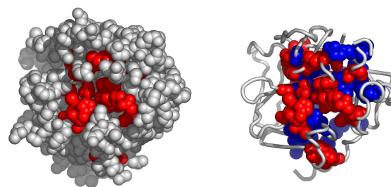
Fig. 11. A possible active surface on the chain 1an1E. The larger cluster it belongs to is shown in blue.
