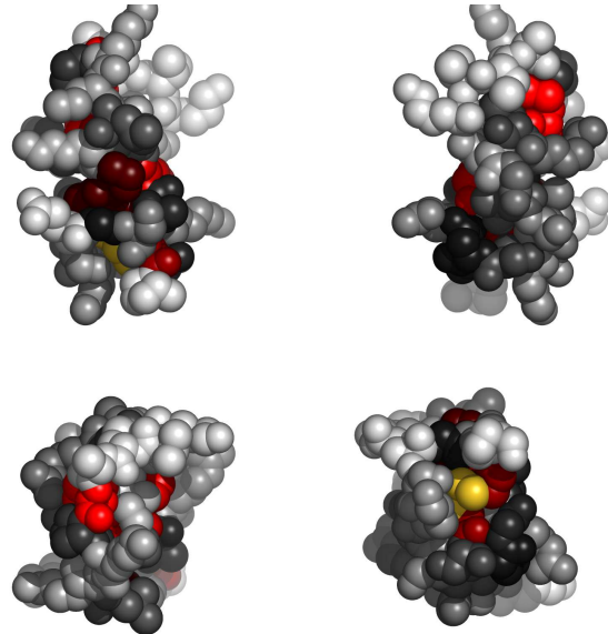
Fig. 2. Residues in 1an1I, colored by their relative importance. Clockwise: front, back, top and bottom views.
