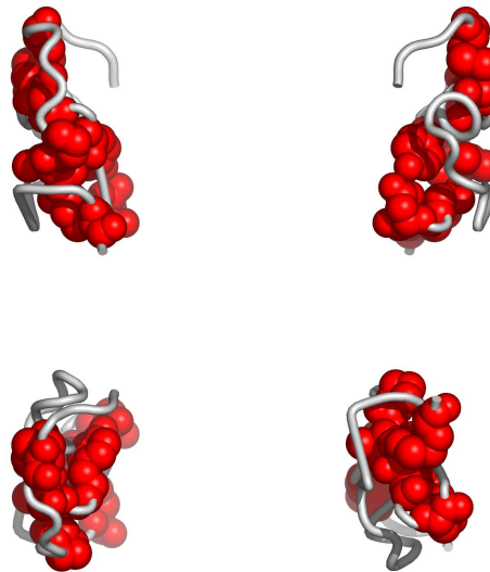
Fig. 2. Residues in 1an1I, colored by their relative importance. Clockwise: front, back, top and bottom views.
