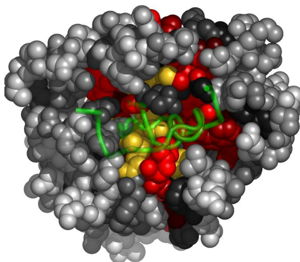
Fig. 10. Residues in 1an1E, at the interface with 1an1I, colored by their relative importance. 1an1I is shown in backbone representation (See Appendix for the coloring scheme for the protein chain 1an1E.)
