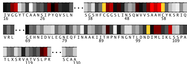
Fig. 6. Residues 16-130 in 1an1E colored by their relative importance. (See Appendix, Fig.12, for the coloring scheme.) Note that some residues in 1an1E carry insertion code.
