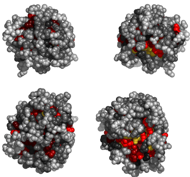
Fig. 8. Residues in 1an1E, colored by their relative importance. Clockwise: front, back, top and bottom views.
