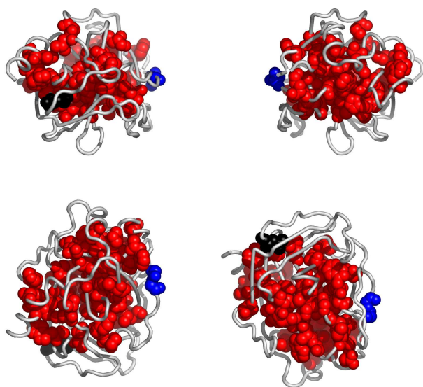
Fig. 9. Residues in 1an1E, colored according to the cluster they belong to: red, followed by blue and yellow are the largest clusters (see Appendix for the coloring scheme). Clockwise: front, back, top and bottom views. The corresponding Pymol script is attached.
