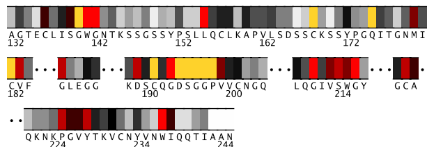
Fig. 7. Residues 132-245 in 1an1E colored by their relative importance. (See Appendix, Fig.12, for the coloring scheme.) Note that some residues in 1an1E carry insertion code.
