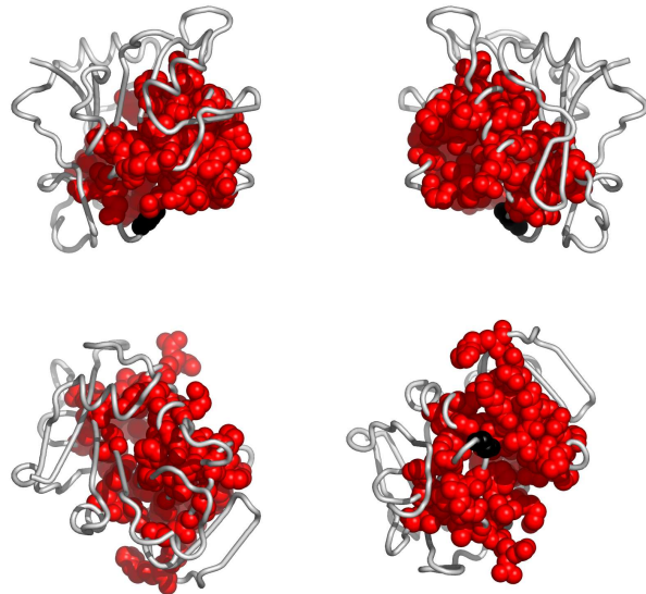
Fig. 3. Residues in laoeA, colored according to the cluster they belong to: red, followed by blue and yellow are the largest clusters (see Appendix for the coloring scheme). Clockwise: front, back, top and bottom views. The corresponding Pymol script is attached.
