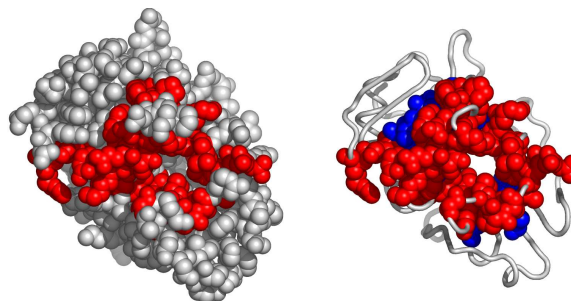
Fig. 6. A possible active surface on the chain laoeA. The larger cluster it belongs to is shown in blue.
