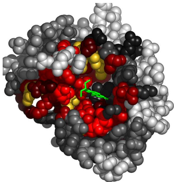
Fig. 4. Residues in 1aoeA, at the interface with GW3, colored by their relative importance. The ligand (GW3) is colored green. Atoms further than 30 Å away from the geometric center of the ligand, as well as on the line of sight to the ligand were removed. (See Appendix for the coloring scheme for the protein chain 1aoeA.)
