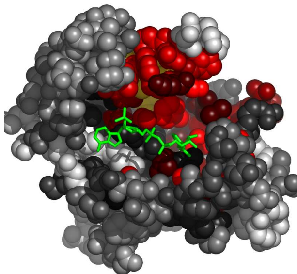
Fig. 5. Residues in laoeA, at the interface with NDP, colored by their relative importance. The ligand (NDP) is colored green. Atoms further than 30Å away from the geometric center of the ligand, as well as on the line of sight to the ligand were removed. (See Appendix for the coloring scheme for the protein chain laoeA.)
