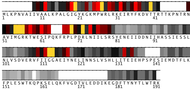
Fig. 1. Residues 1-192 in laoeA colored by their relative importance. (See Appendix, Fig.7, for the coloring scheme.)
