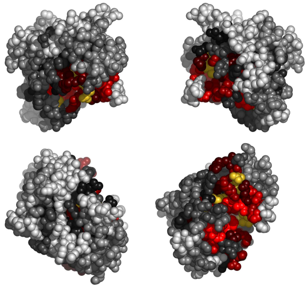
Fig. 2. Residues in laoeA, colored by their relative importance. Clockwise: front, back, top and bottom views.
