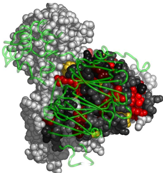
Fig. 6. Residues in 1aofB, at the interface with 1aofA, colored by their relative importance. 1aofA is shown in backbone representation (See Appendix for the coloring scheme for the protein chain 1aofB.)
