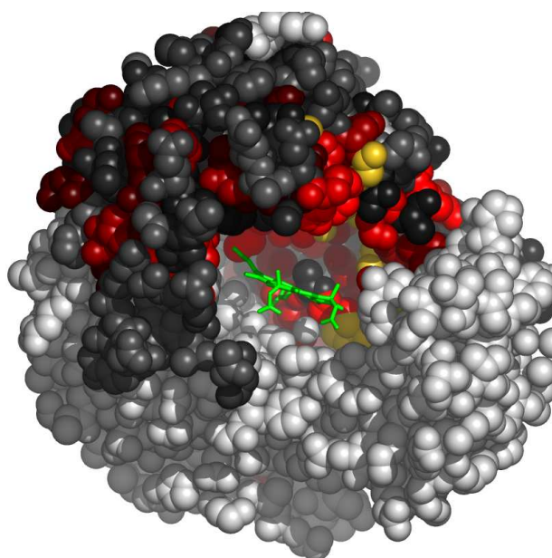
Fig. 5. Residues in 1aofB, at the interface with heme d, colored by their relative importance. The ligand (heme d) is colored green. Atoms further than 30 Å away from the geometric center of the ligand, as well as on the line of sight to the ligand were removed. (See Appendix for the coloring scheme for the protein chain 1aofB.)
