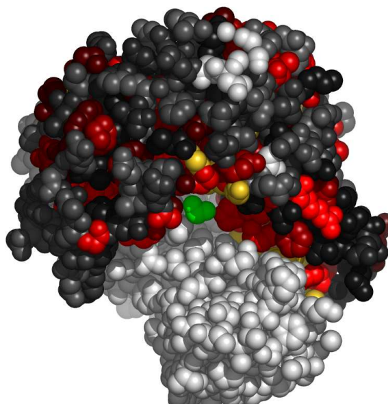
Fig. 7. Residues in 1aofB, at the interface with sulfur dioxide, colored by their relative importance. The ligand (sulfur dioxide) is colored green. Atoms further than 30 Å away from the geometric center of the ligand, as well as on the line of sight to the ligand were removed. (See Appendix for the coloring scheme for the protein chain 1aofB.)
