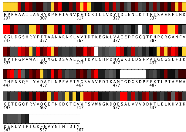
Fig. 2. Residues 297-567 in 1aofB colored by their relative importance. (See Appendix, Fig.8, for the coloring scheme.)
