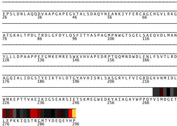
Fig. 1. Residues 26-296 in 1aofB colored by their relative importance. (See Appendix, Fig.8, for the coloring scheme.)
