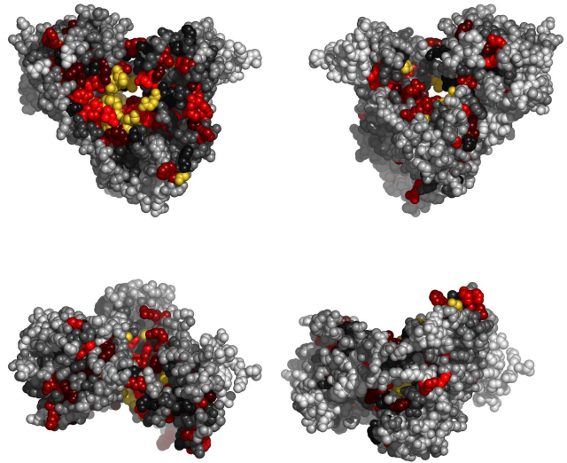
Fig. 3. Residues in 1aogA, colored by their relative importance. Clockwise: front, back, top and bottom views.
