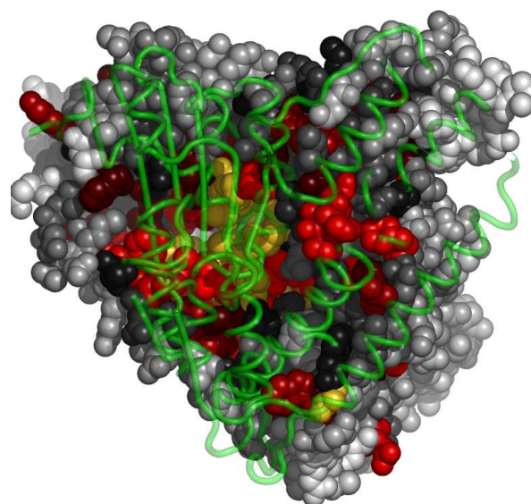
Fig. 6. Residues in IaogA, at the interface with IaogB, colored by their relative importance. IaogB is shown in backbone representation (See Appendix for the coloring scheme for the protein chain IaogA.)
