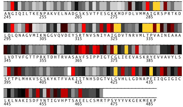
Fig. 2. Residues 245-487 in 1aogA colored by their relative importance. (See Appendix, Fig.10, for the coloring scheme.)
