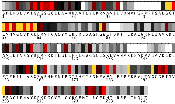
Fig. 1. Residues 3-244 in 1aogA colored by their relative importance. (See Appendix, Fig.10, for the coloring scheme.)
