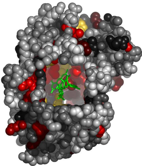
Fig. 5. Residues in 1aogA, at the interface with FAD, colored by their relative importance. The ligand (FAD) is colored green. Atoms further than 30Å away from the geometric center of the ligand, as well as on the line of sight to the ligand were removed. (See Appendix for the coloring scheme for the protein chain 1aogA.)
