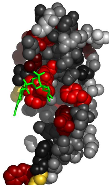
Fig. 8. Residues in 1aogA, at the interface with FAD, colored by their relative importance. The ligand (FAD) is colored green. Atoms further than 30\text{\AA} away from the geometric center of the ligand, as well as on the line of sight to the ligand were removed. (See Appendix for the coloring scheme for the protein chain 1aogA.)
