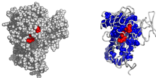
Fig. 9. A possible active surface on the chain 1aogA. The larger cluster it belongs to is shown in blue.
